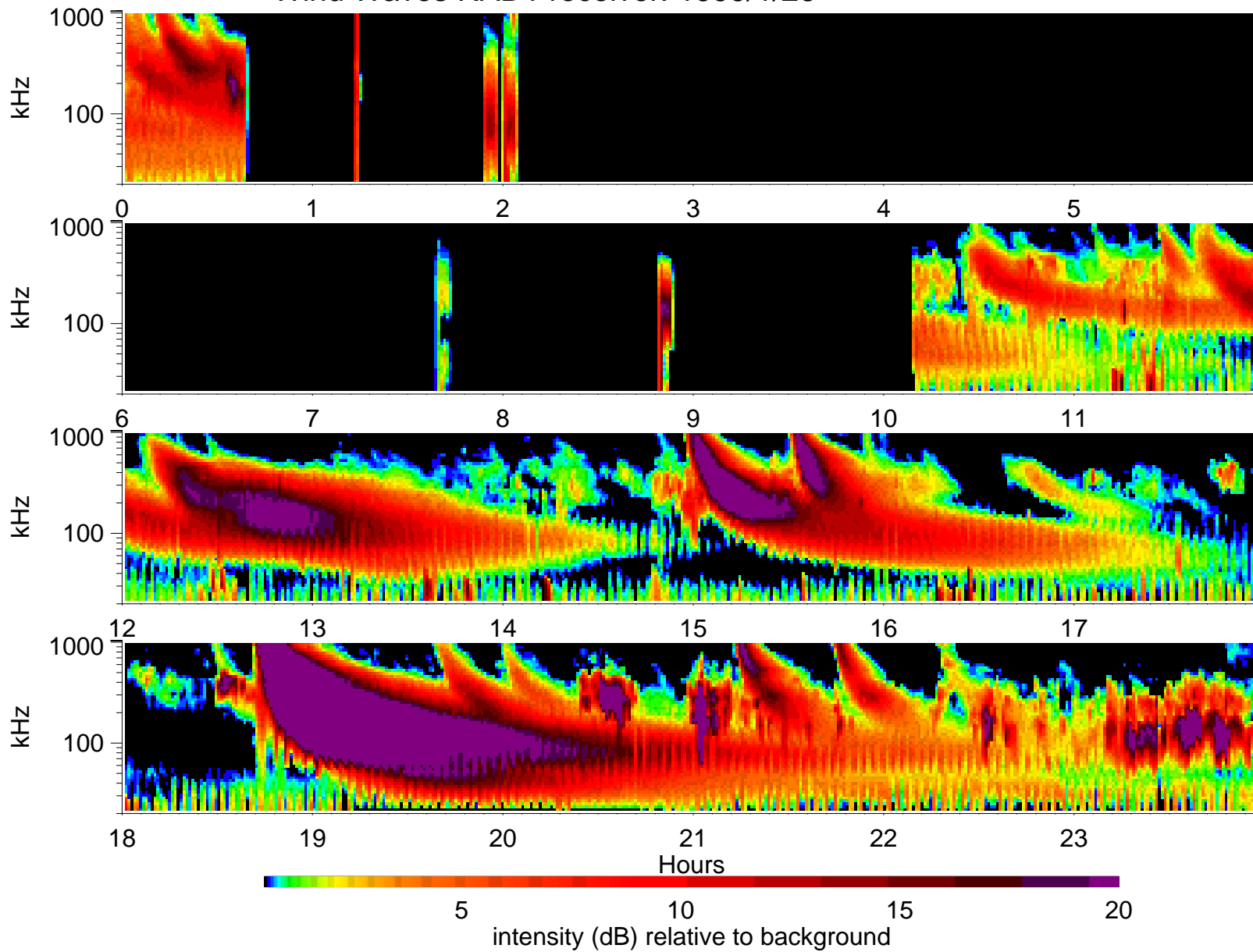
Wind Waves RAD1 receiver: 1999/1/26
