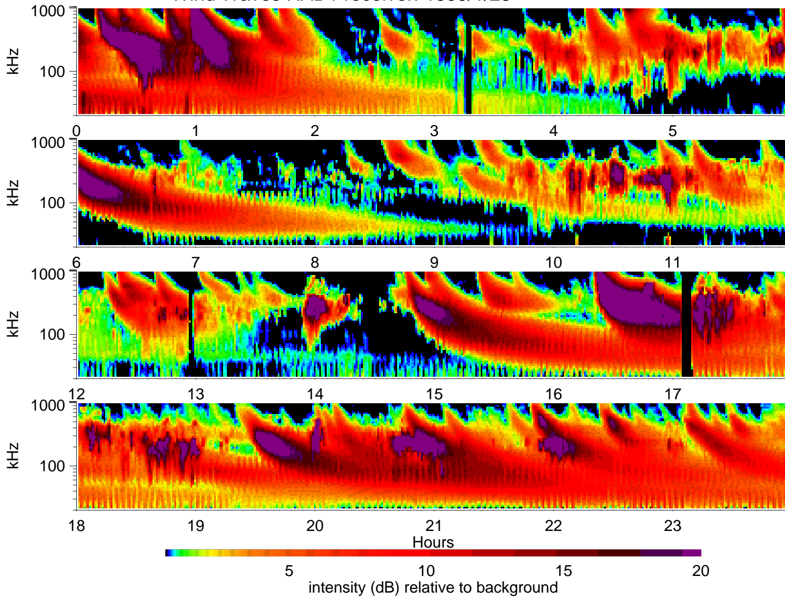
Wind Waves RAD1 receiver: 1999/1/25
