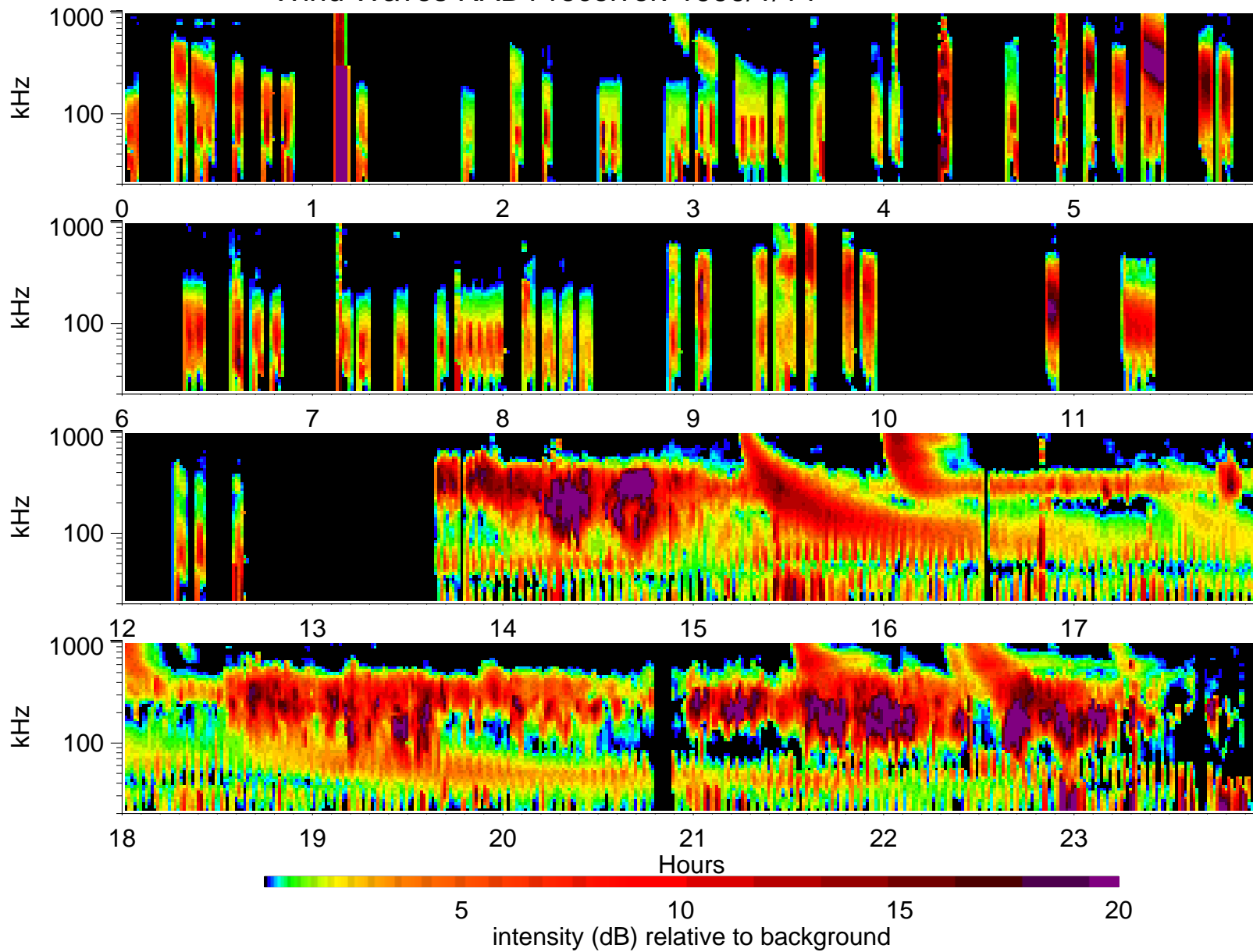
Wind Waves RAD1 receiver: 1999/1/14
