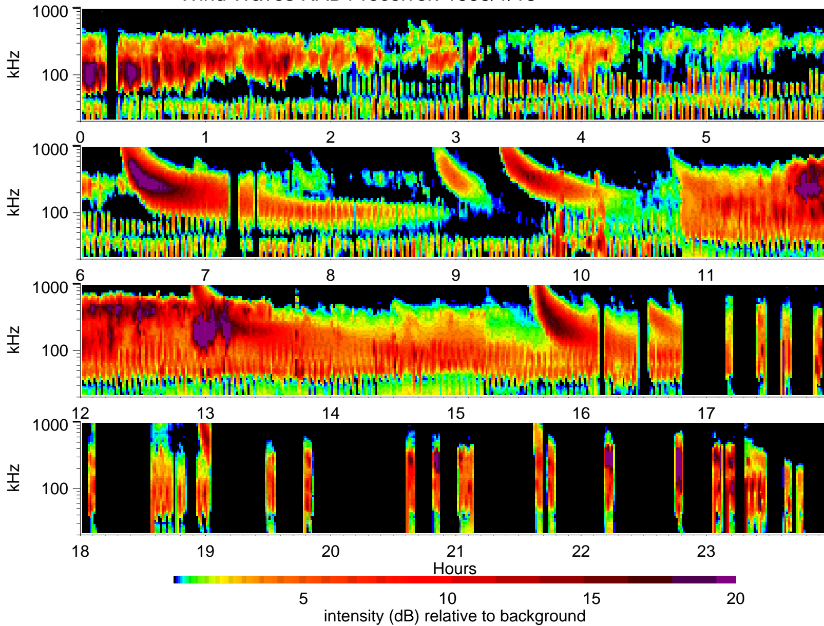
Wind Waves RAD1 receiver: 1999/1/13
