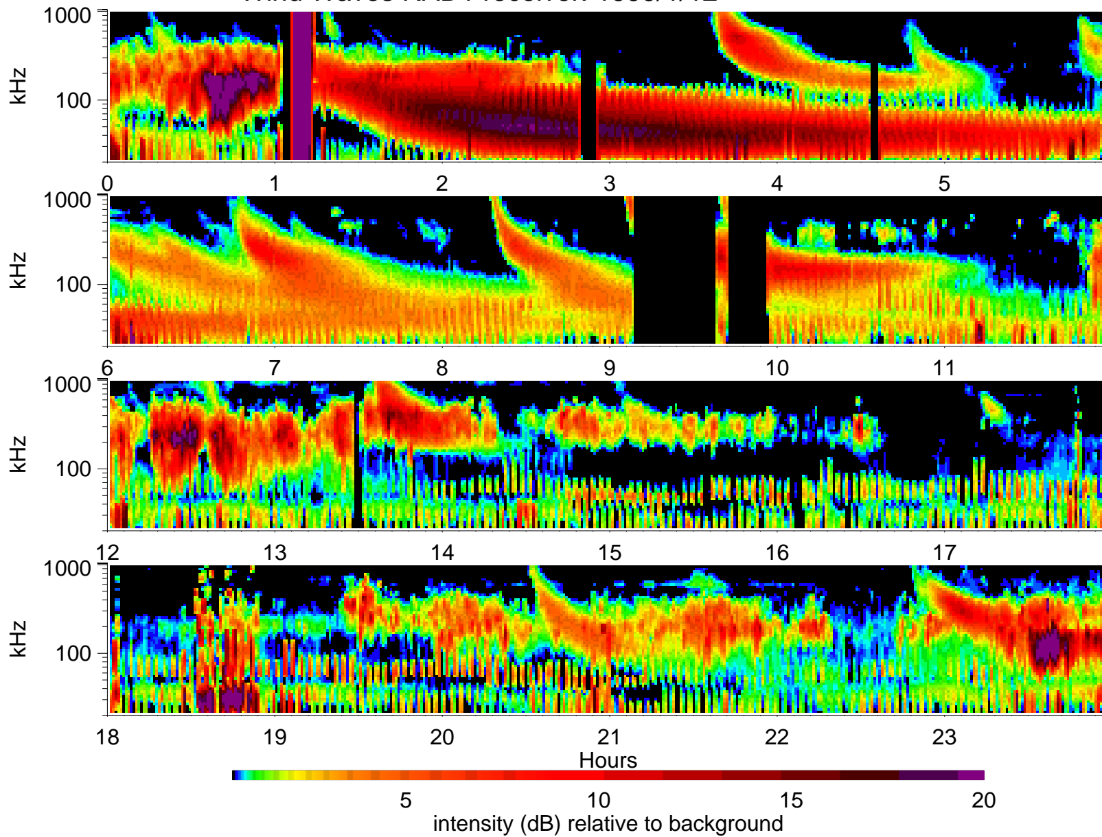
Wind Waves RAD1 receiver: 1999/1/12
