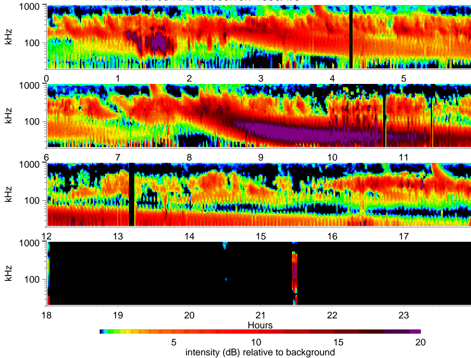
Wind Waves RAD1 receiver: 1999/1/9
