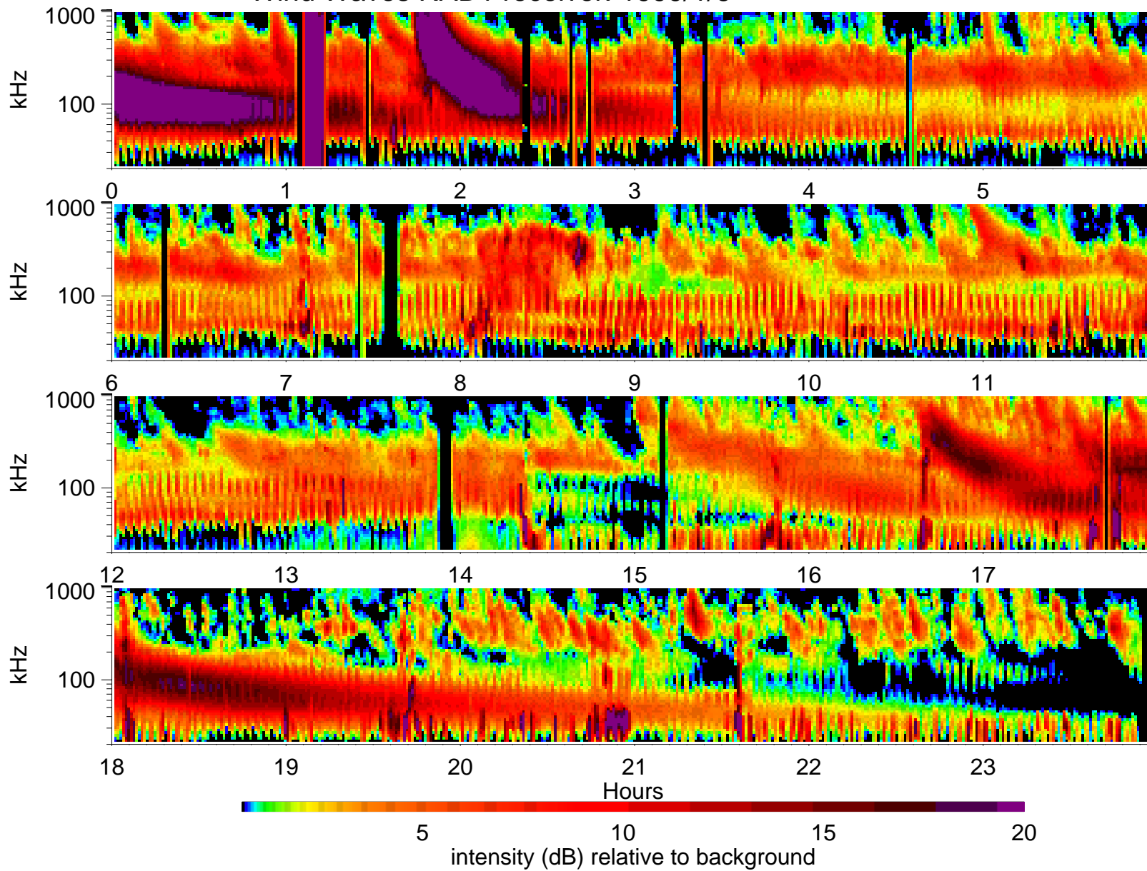
Wind Waves RAD1 receiver: 1999/1/6
