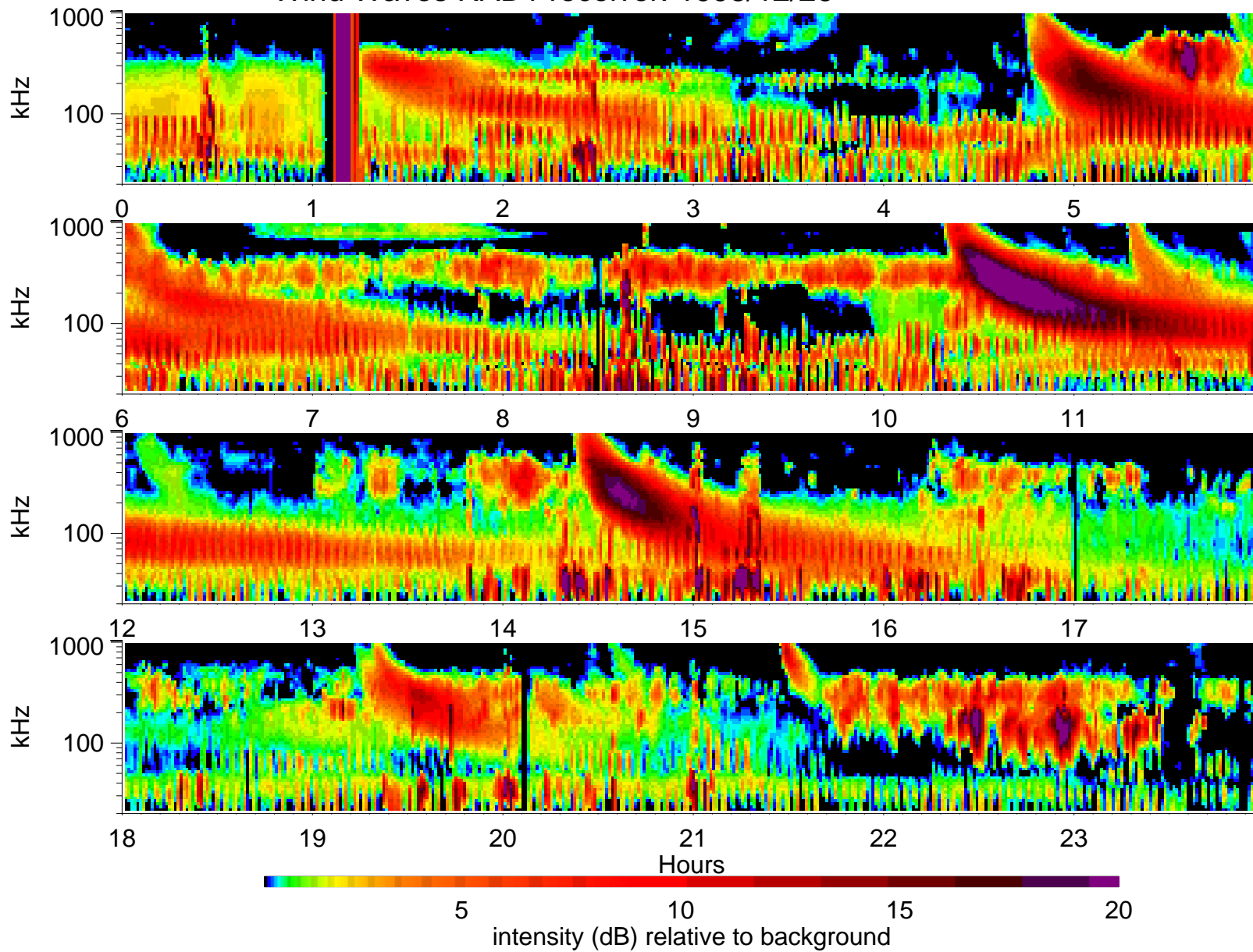
Wind Waves RAD1 receiver: 1998/12/26
