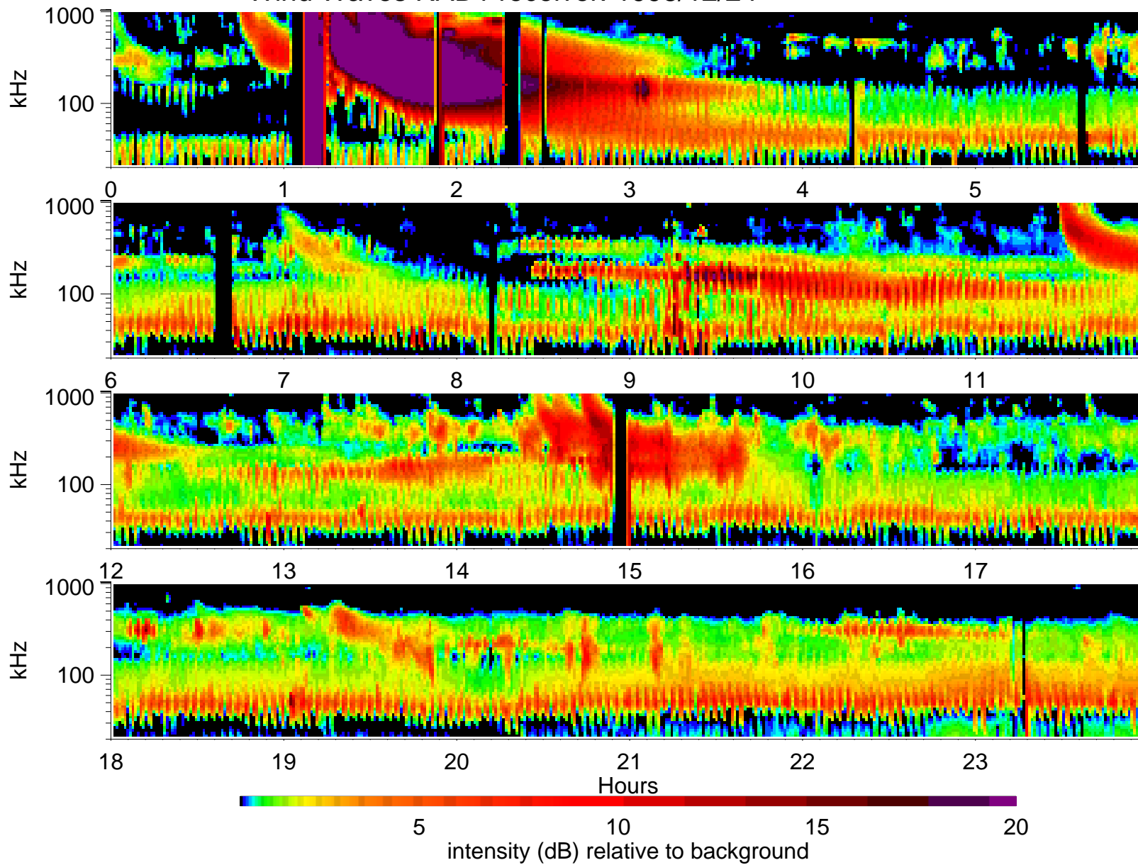
Wind Waves RAD1 receiver: 1998/12/24
