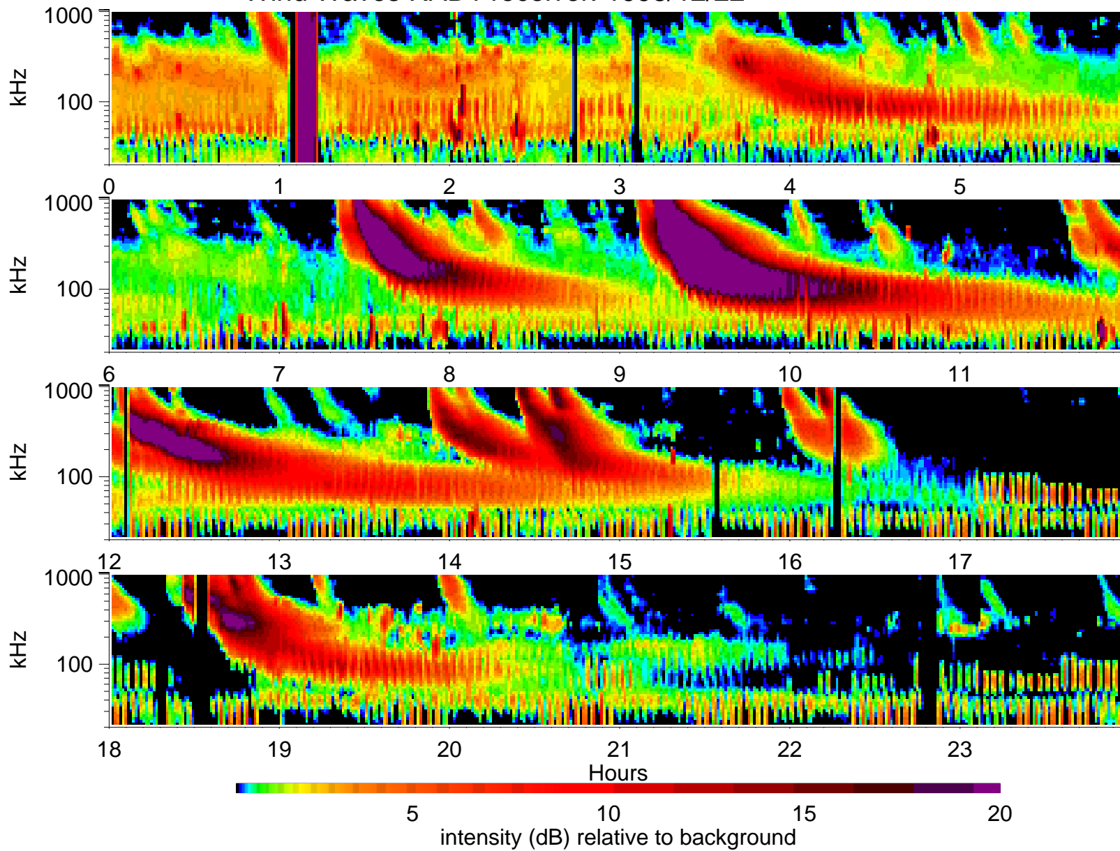
Wind Waves RAD1 receiver: 1998/12/22
