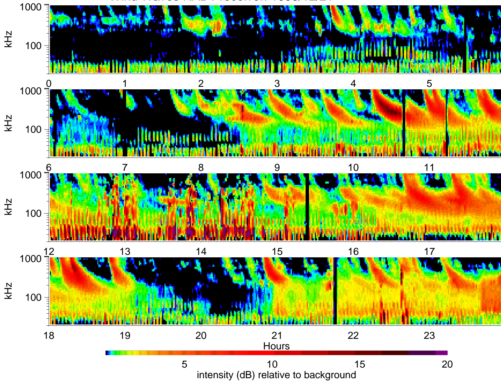
Wind Waves RAD1 receiver: 1998/12/21
