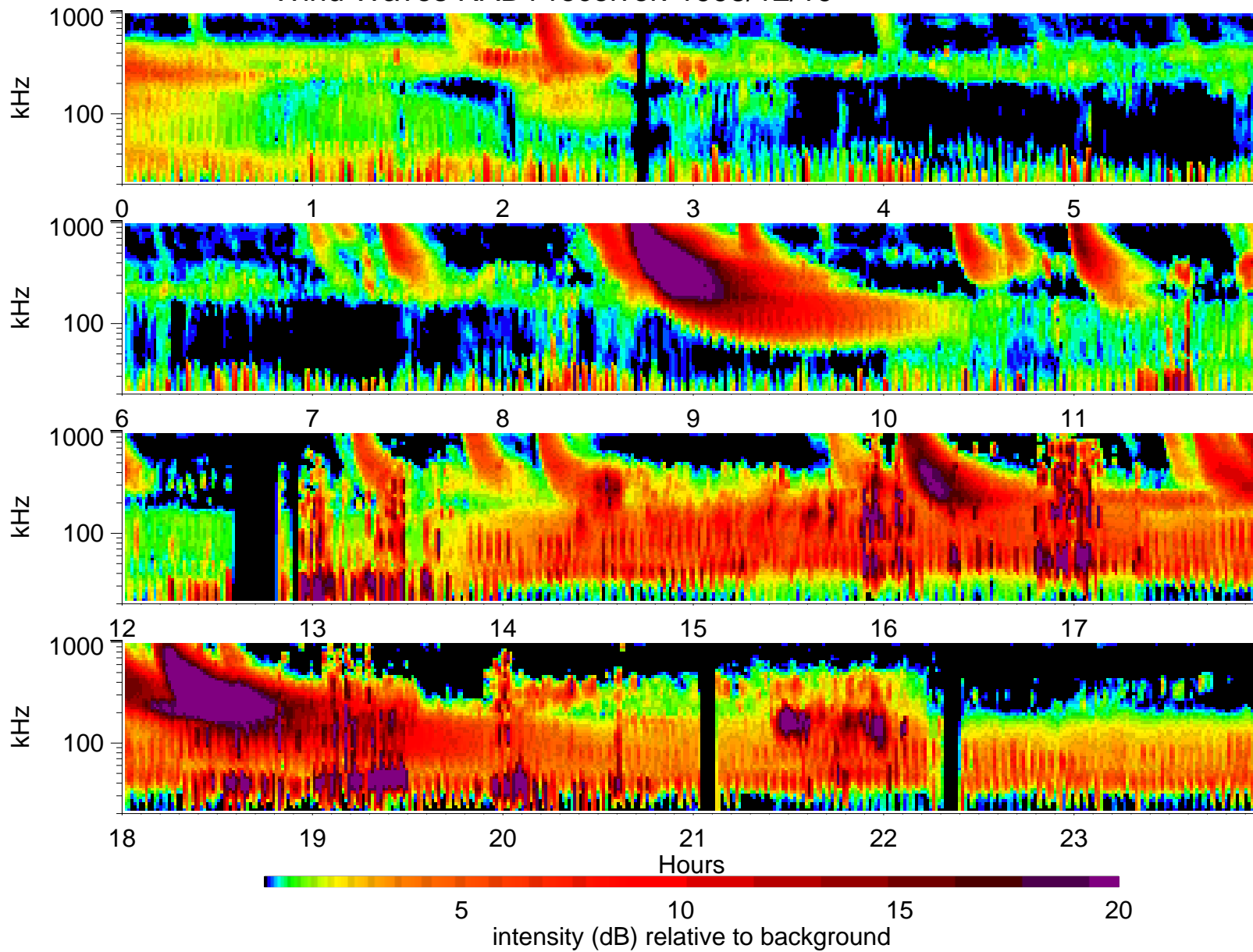
Wind Waves RAD1 receiver: 1998/12/19
