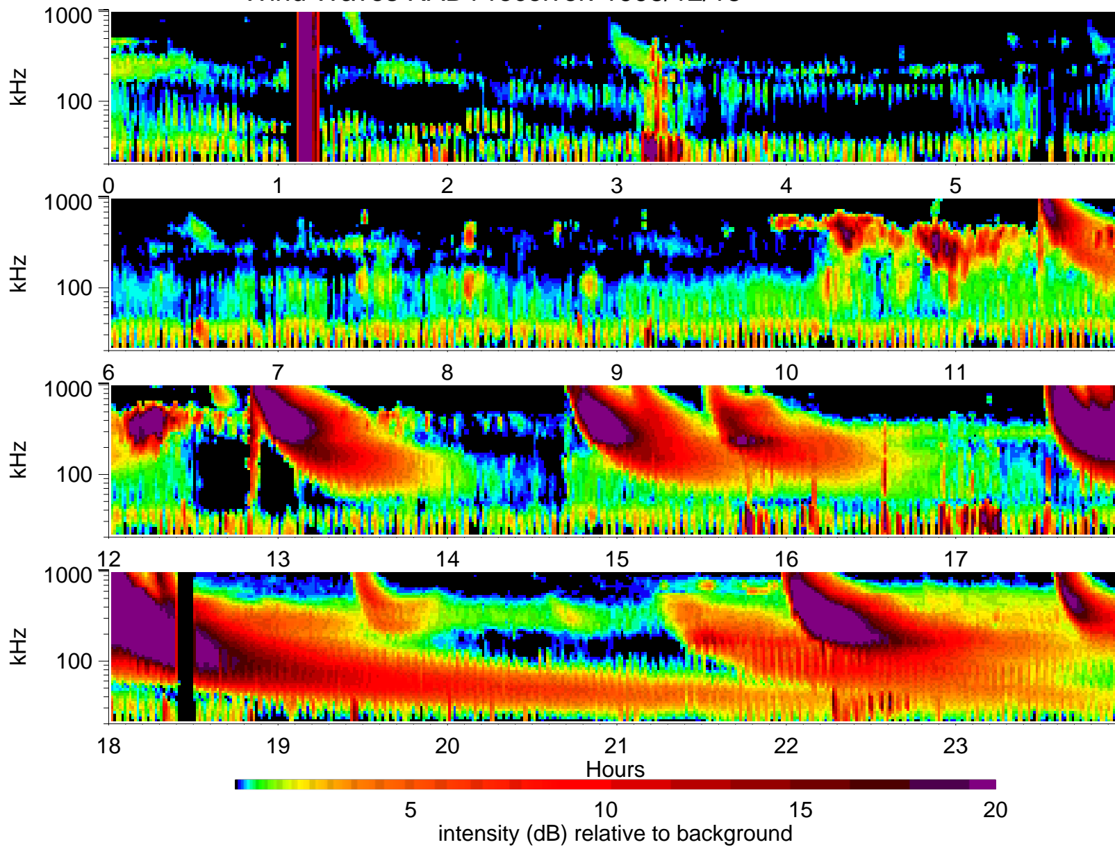
Wind Waves RAD1 receiver: 1998/12/18
