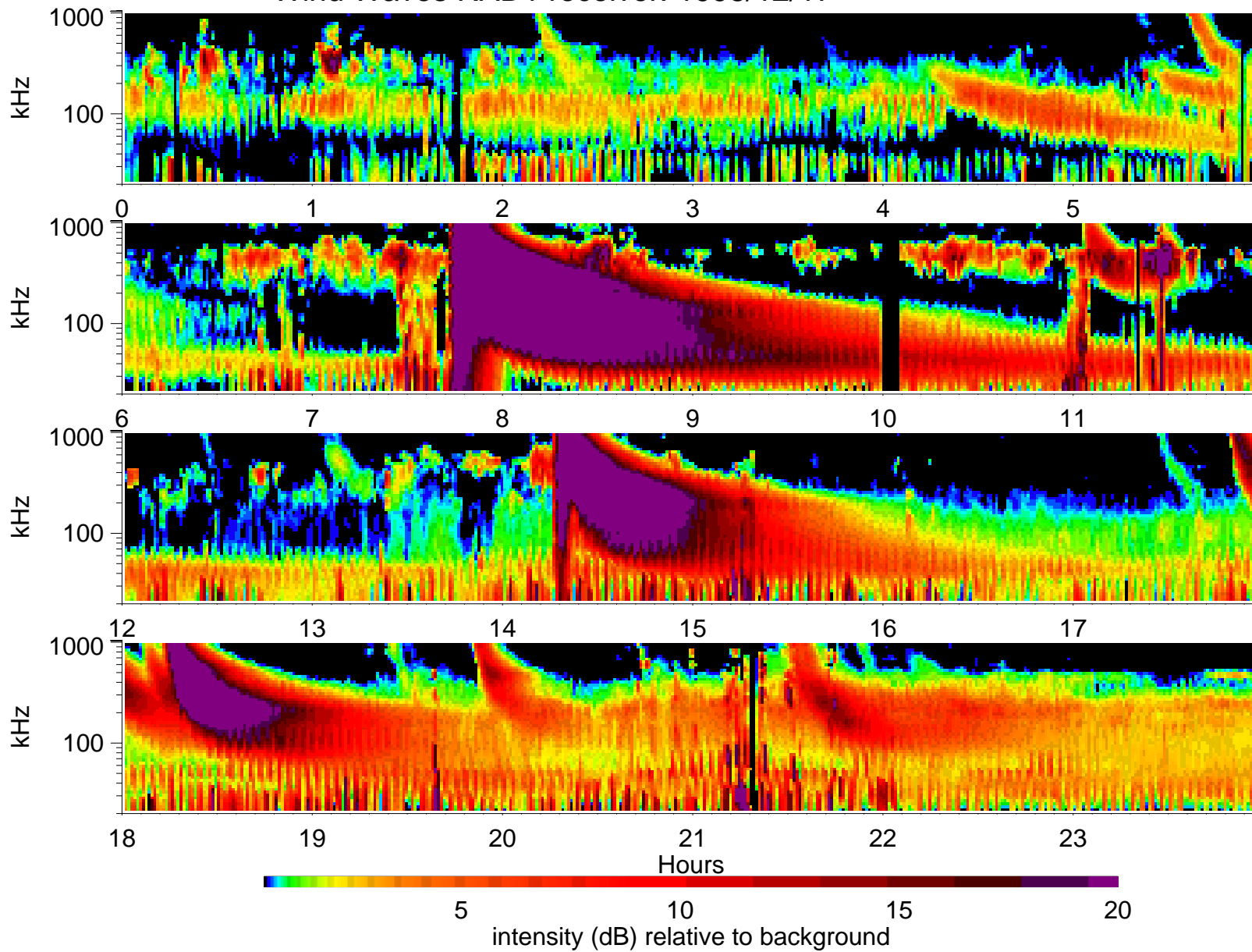
Wind Waves RAD1 receiver: 1998/12/17
