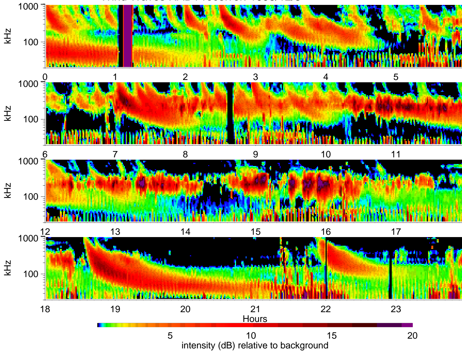
Wind Waves RAD1 receiver: 1998/12/8
