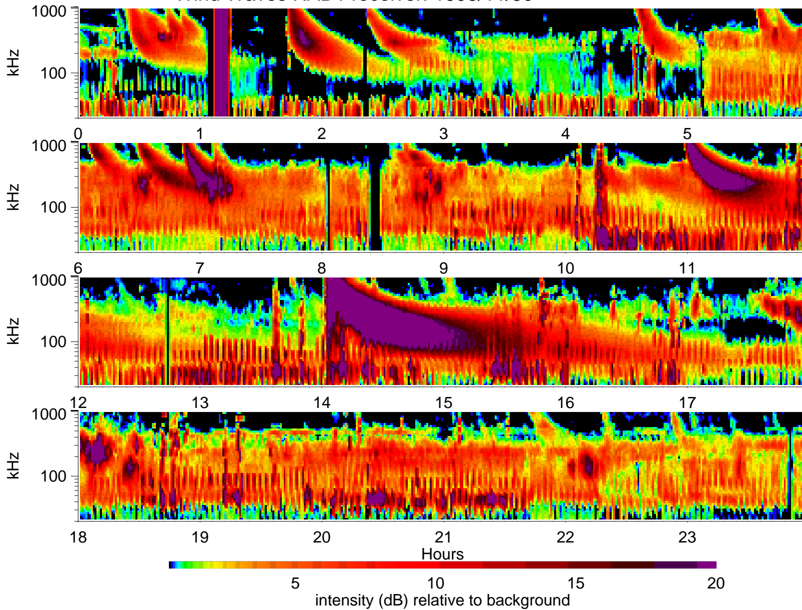
Wind Waves RAD1 receiver: 1998/11/30
