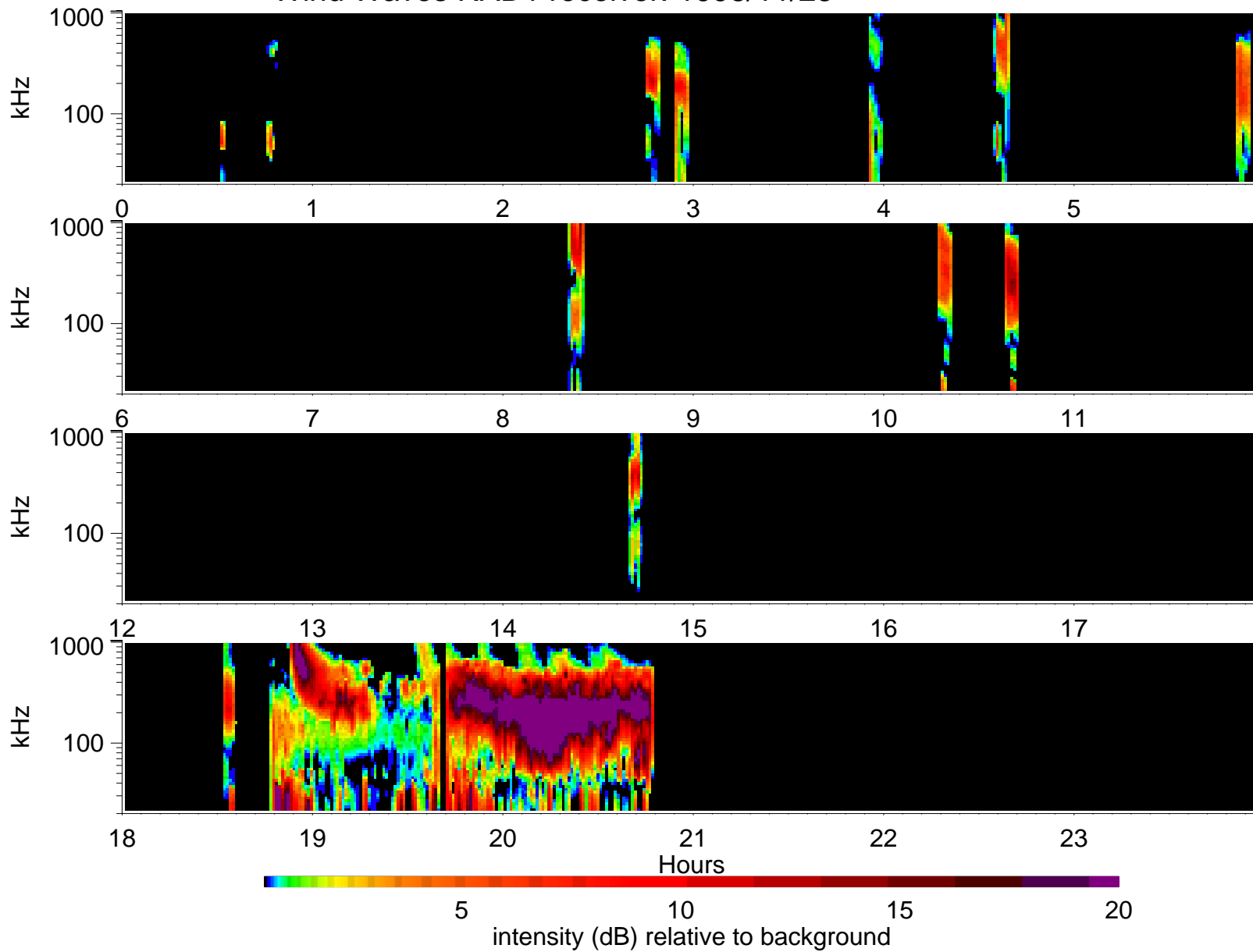
Wind Waves RAD1 receiver: 1998/11/25
