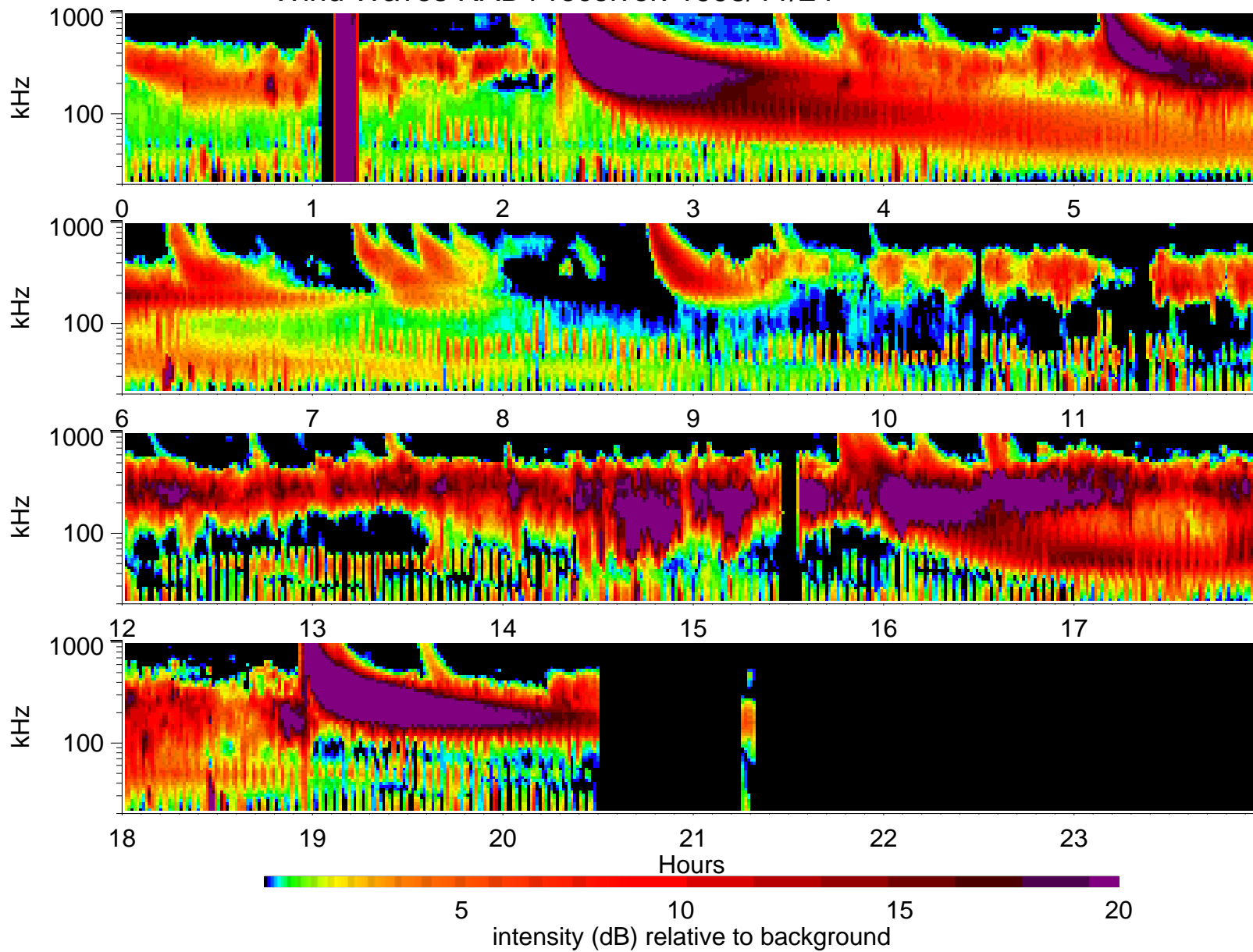
Wind Waves RAD1 receiver: 1998/11/24
