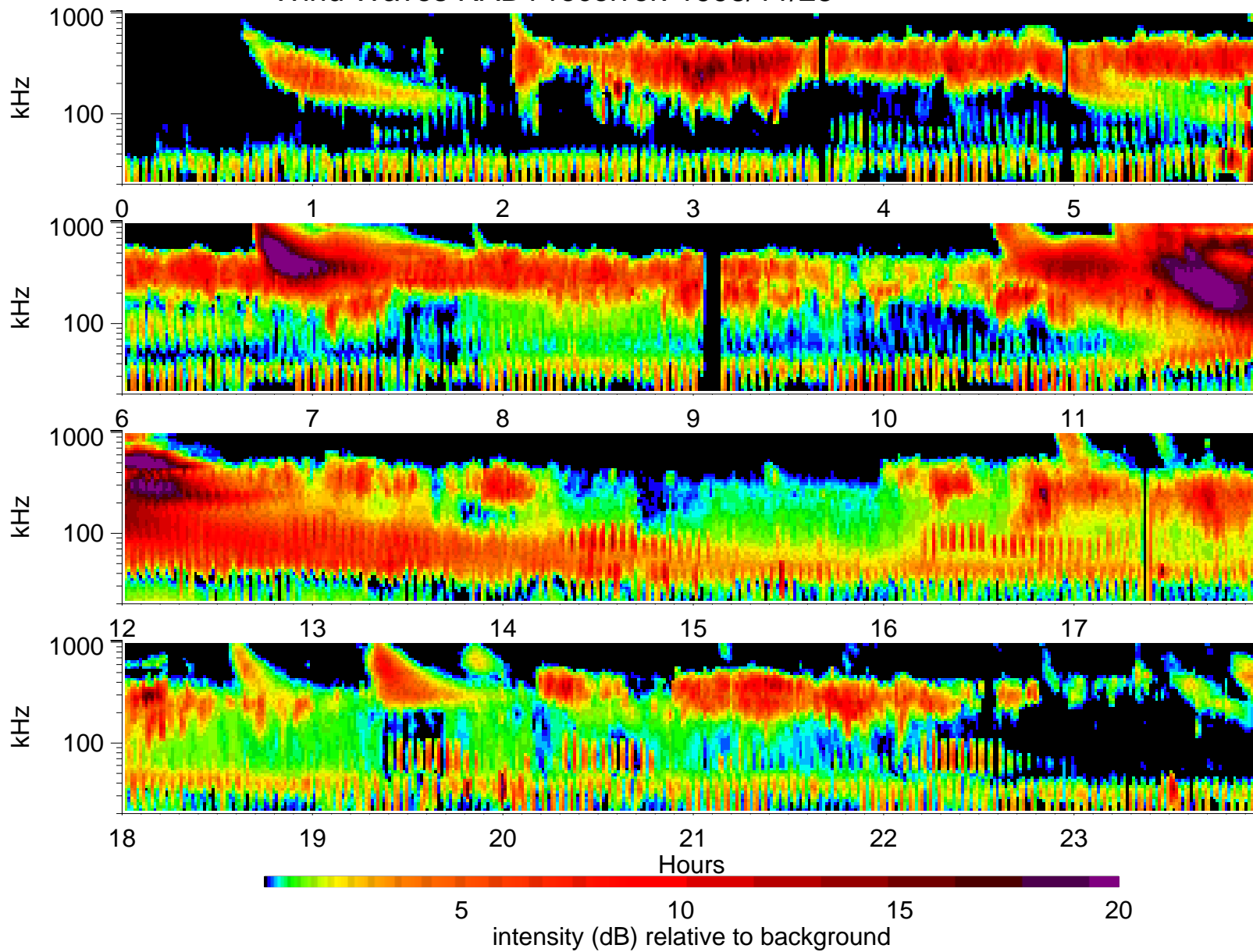
Wind Waves RAD1 receiver: 1998/11/23
