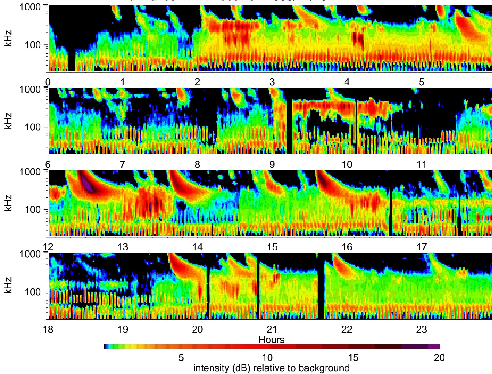
Wind Waves RAD1 receiver: 1998/11/19
