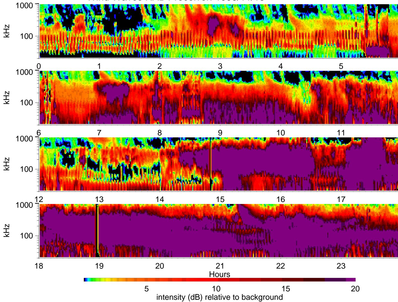
Wind Waves RAD1 receiver: 1998/11/13
