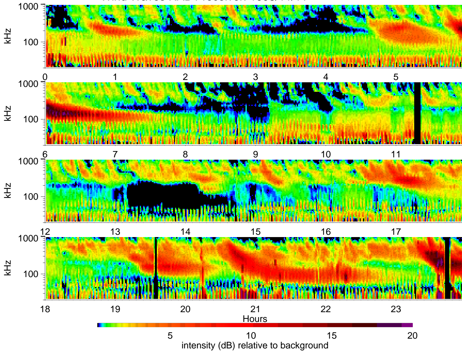
Wind Waves RAD1 receiver: 1998/11/11
