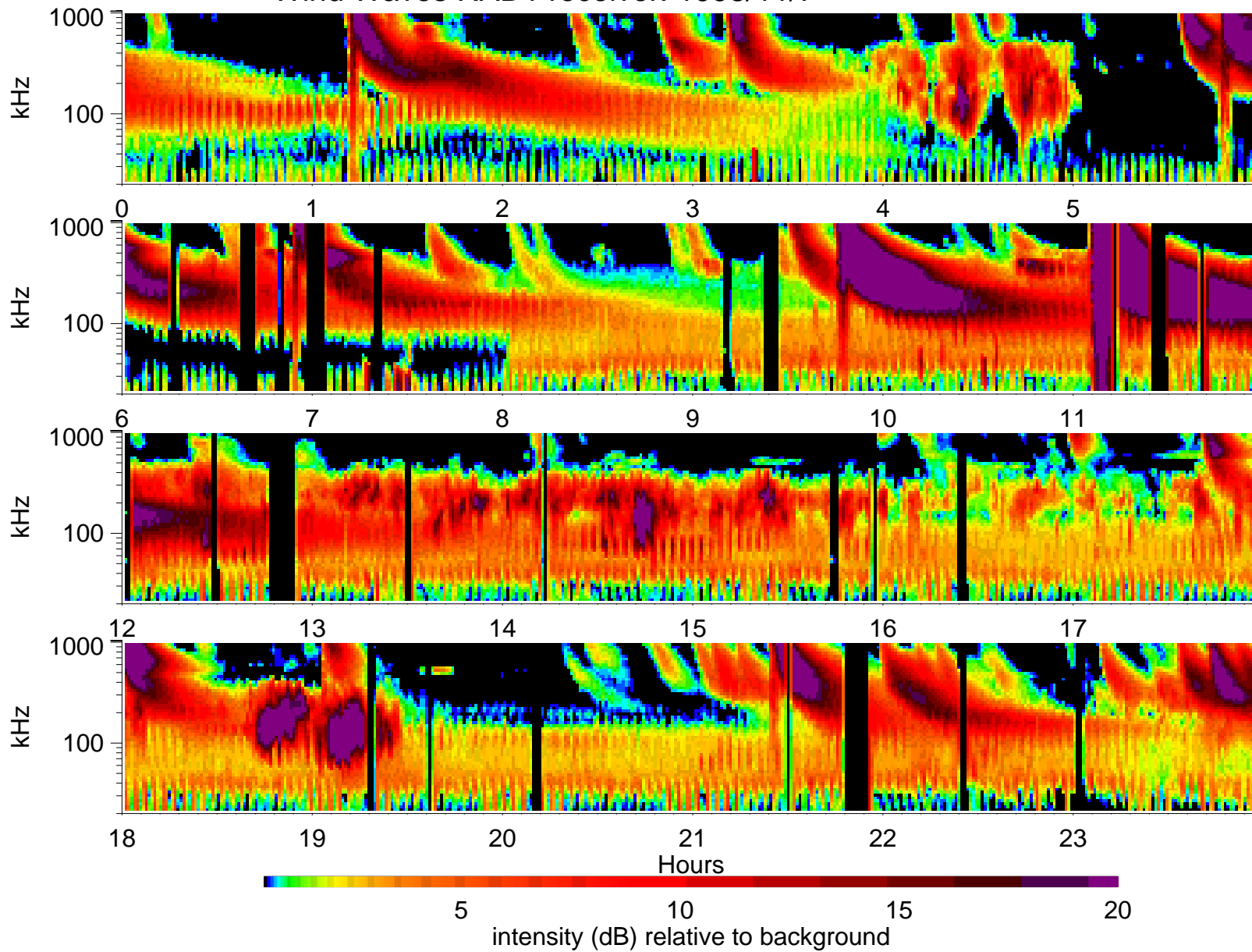
Wind Waves RAD1 receiver: 1998/11/7
