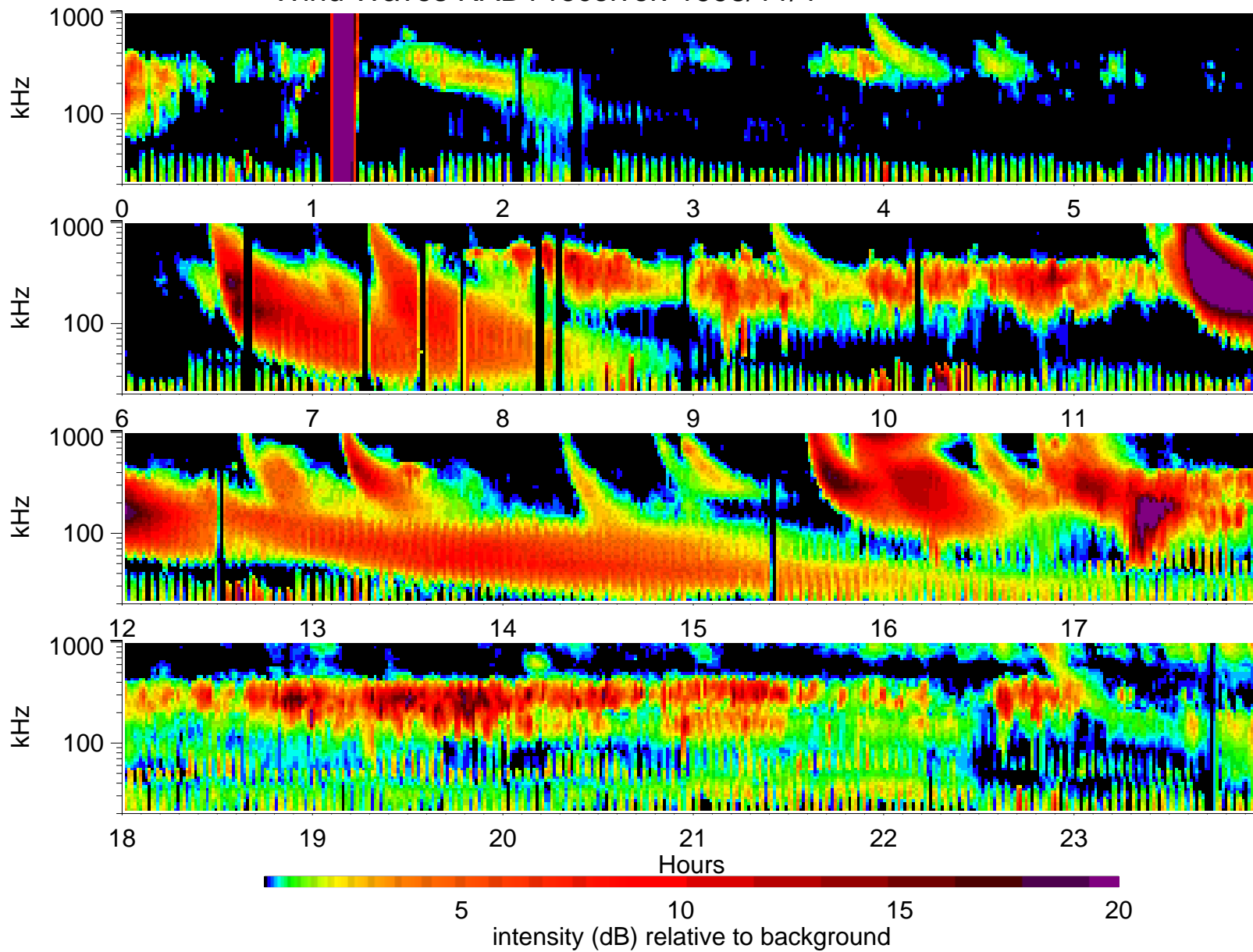
Wind Waves RAD1 receiver: 1998/11/4
