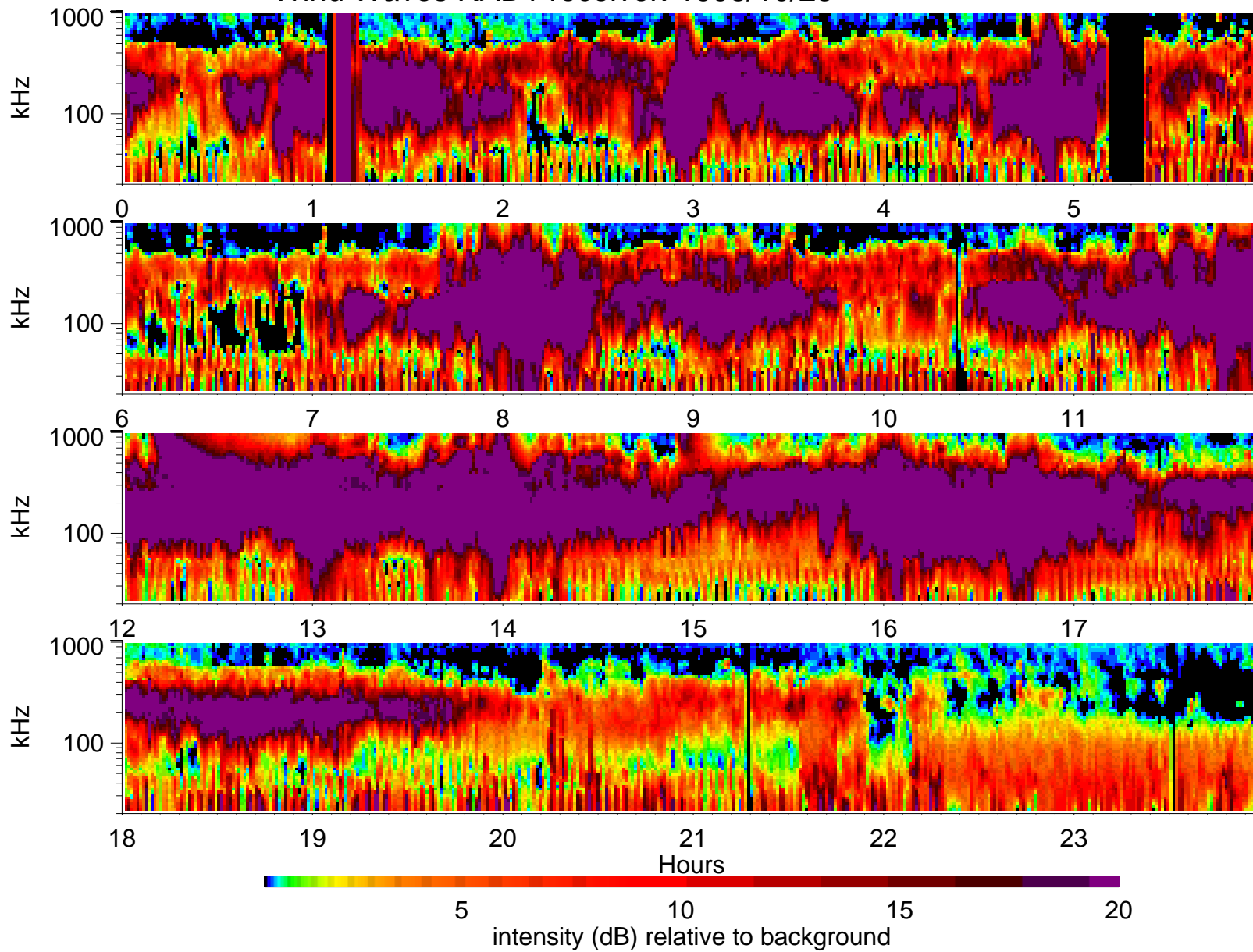
Wind Waves RAD1 receiver: 1998/10/25
