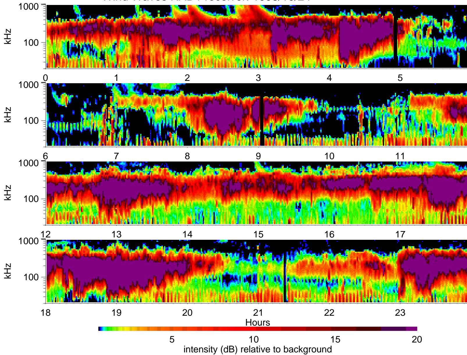
Wind Waves RAD1 receiver: 1998/10/24
