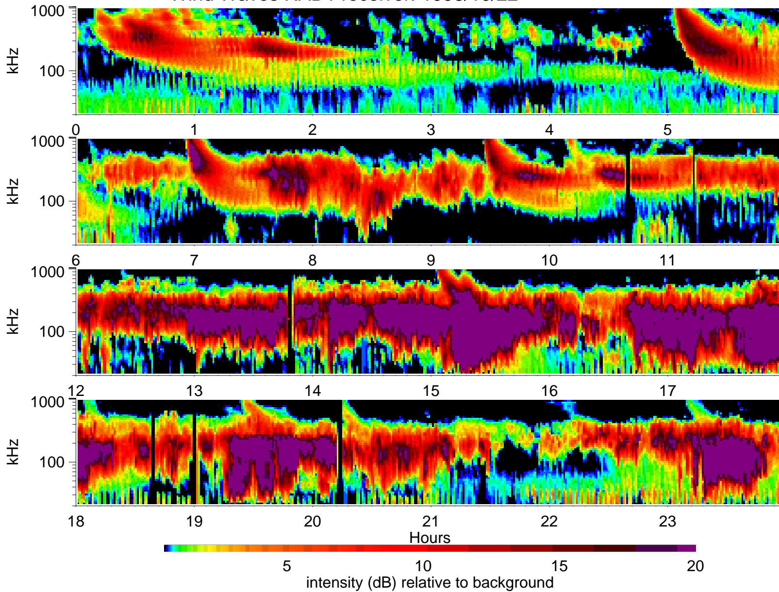
Wind Waves RAD1 receiver: 1998/10/22
