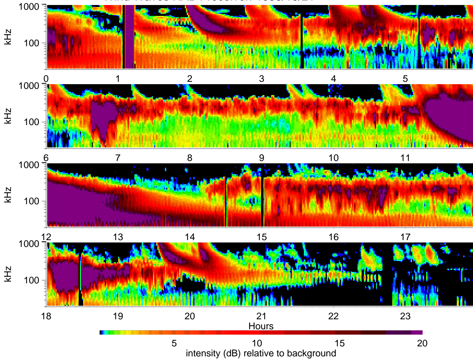
Wind Waves RAD1 receiver: 1998/10/21
