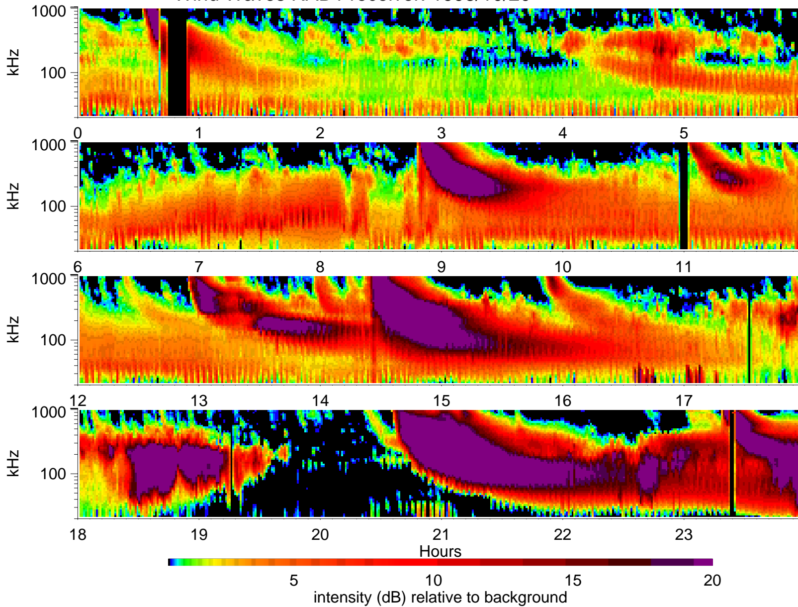
Wind Waves RAD1 receiver: 1998/10/20
