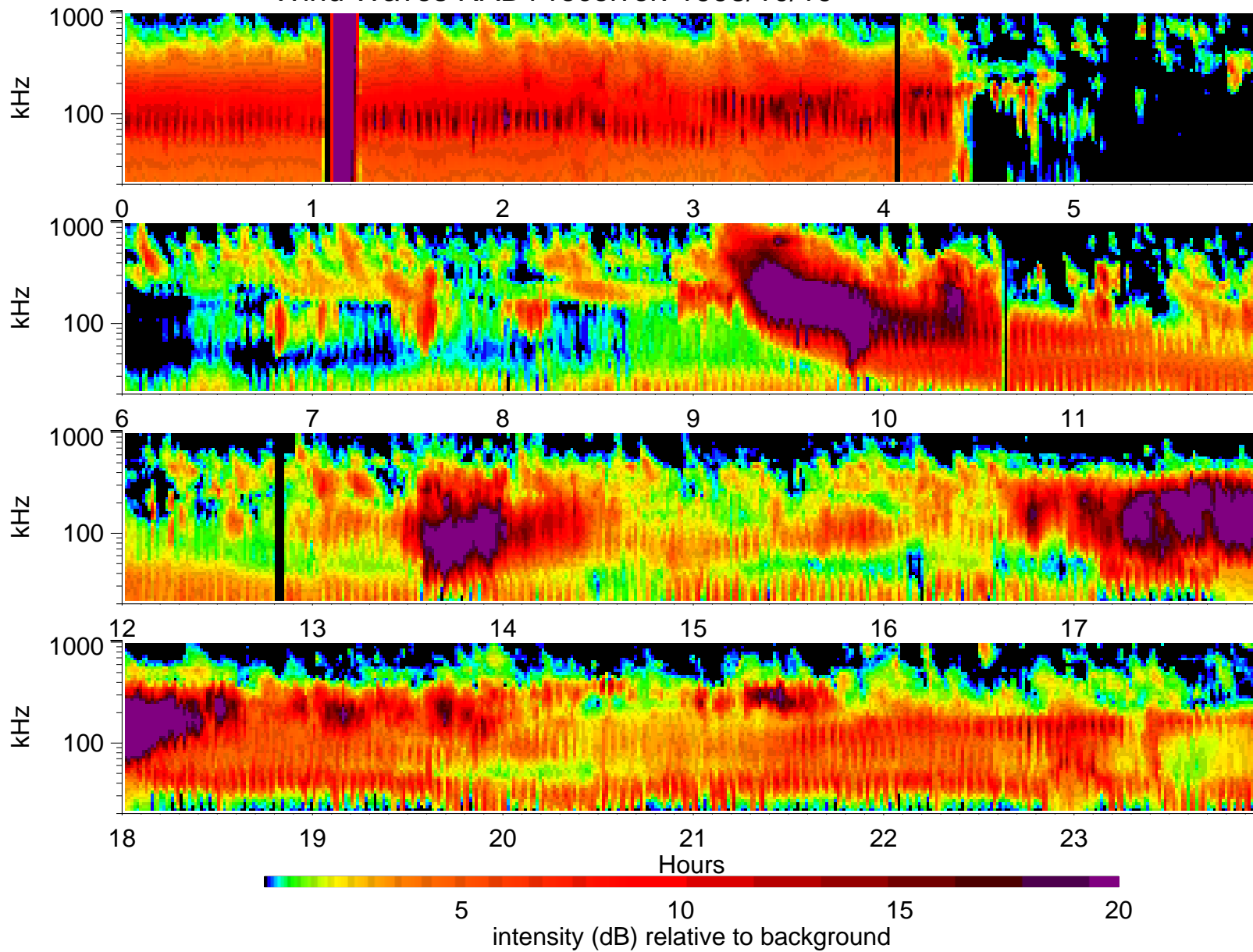
Wind Waves RAD1 receiver: 1998/10/19
