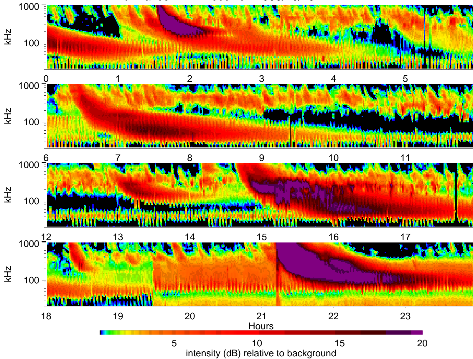
Wind Waves RAD1 receiver: 1998/10/18
