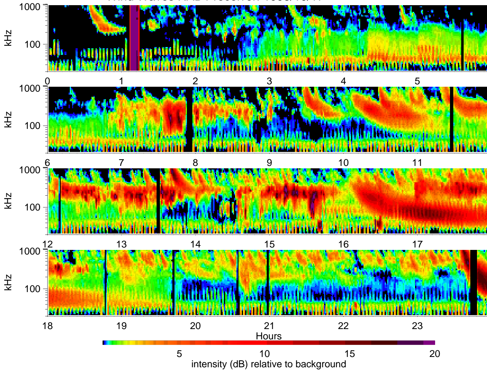
Wind Waves RAD1 receiver: 1998/10/17
