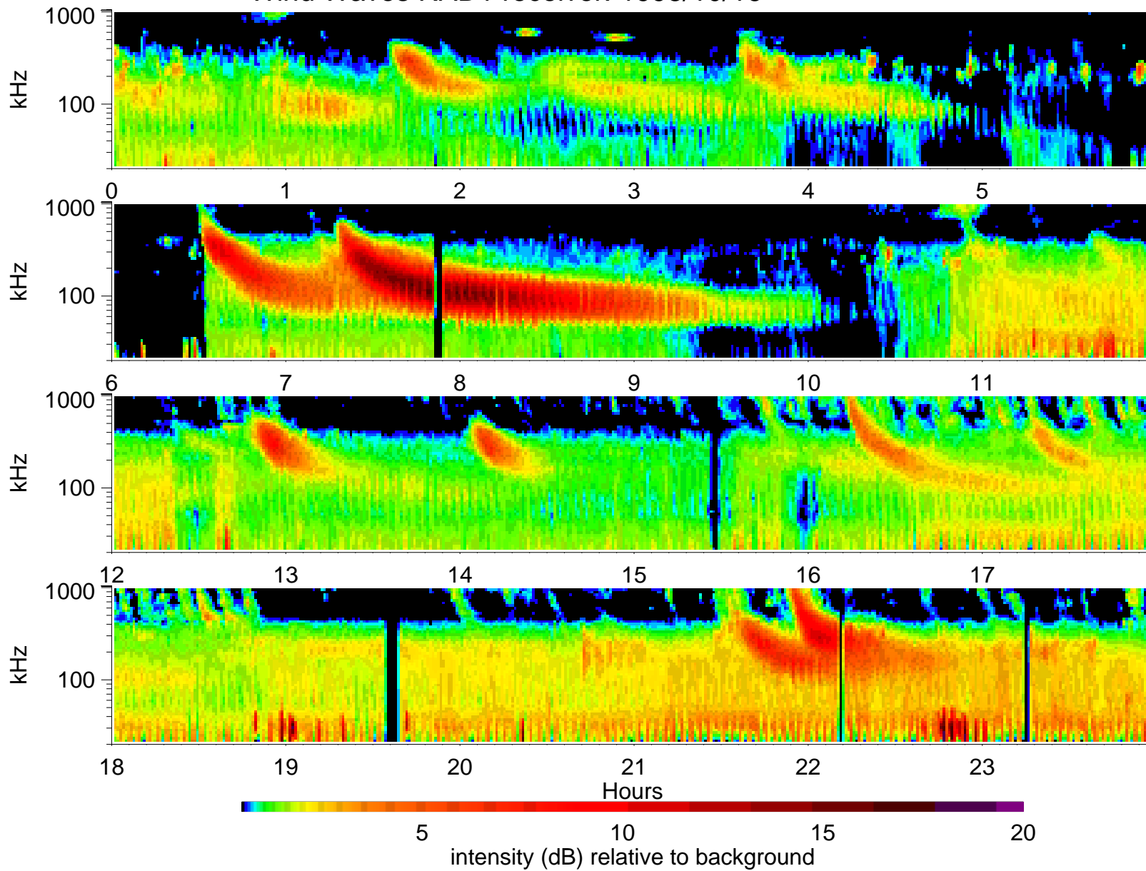
Wind Waves RAD1 receiver: 1998/10/16
