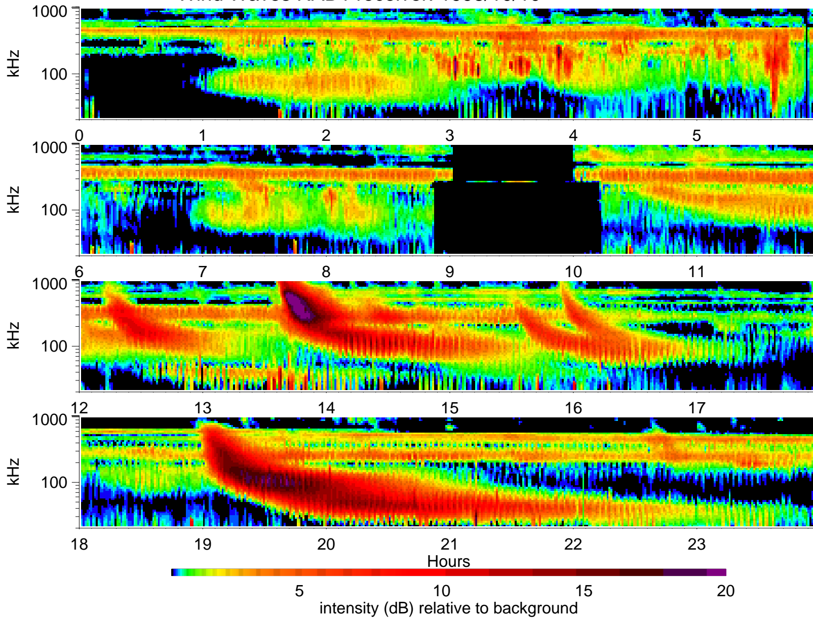
Wind Waves RAD1 receiver: 1998/10/10
