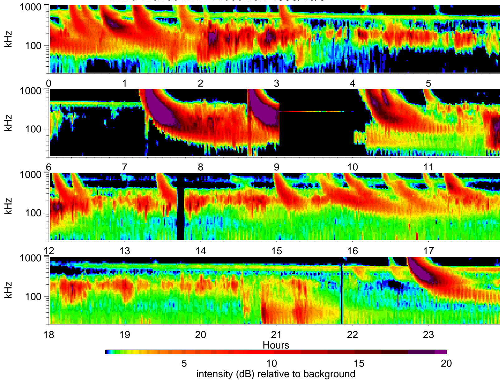
Wind Waves RAD1 receiver: 1998/10/8
