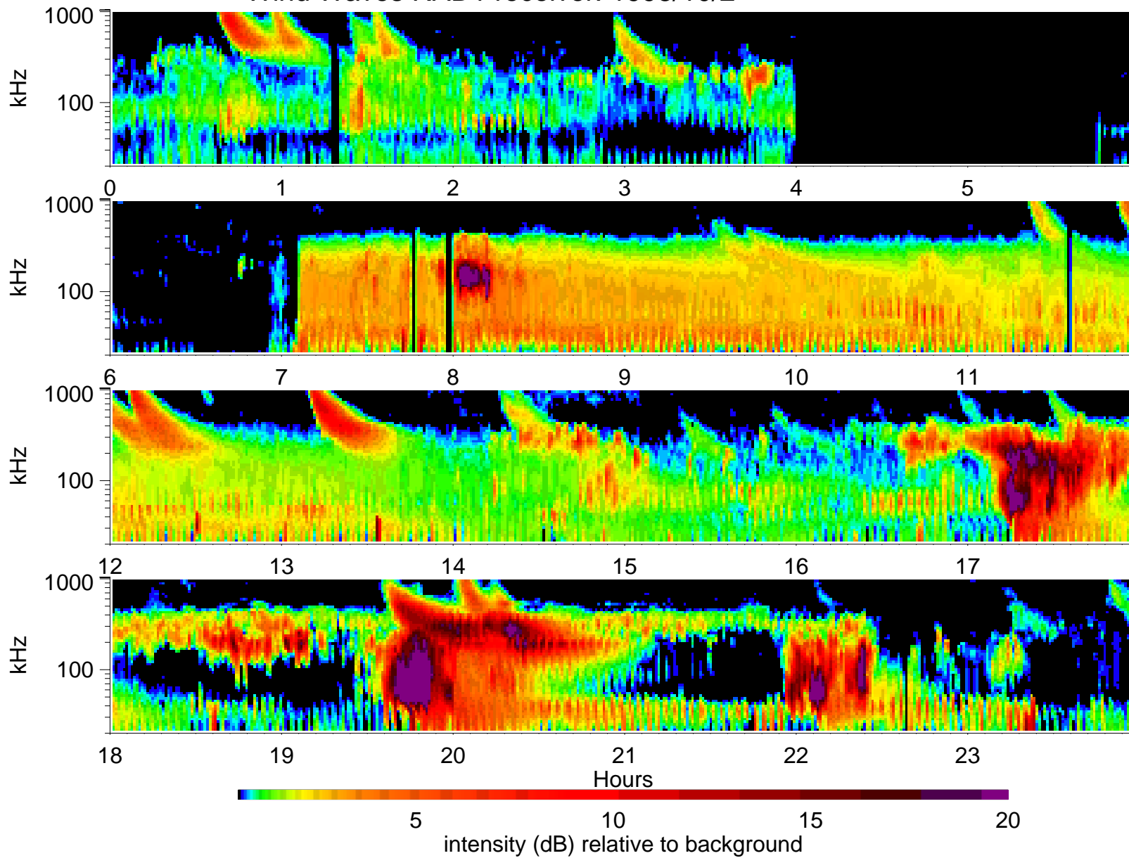
Wind Waves RAD1 receiver: 1998/10/2
