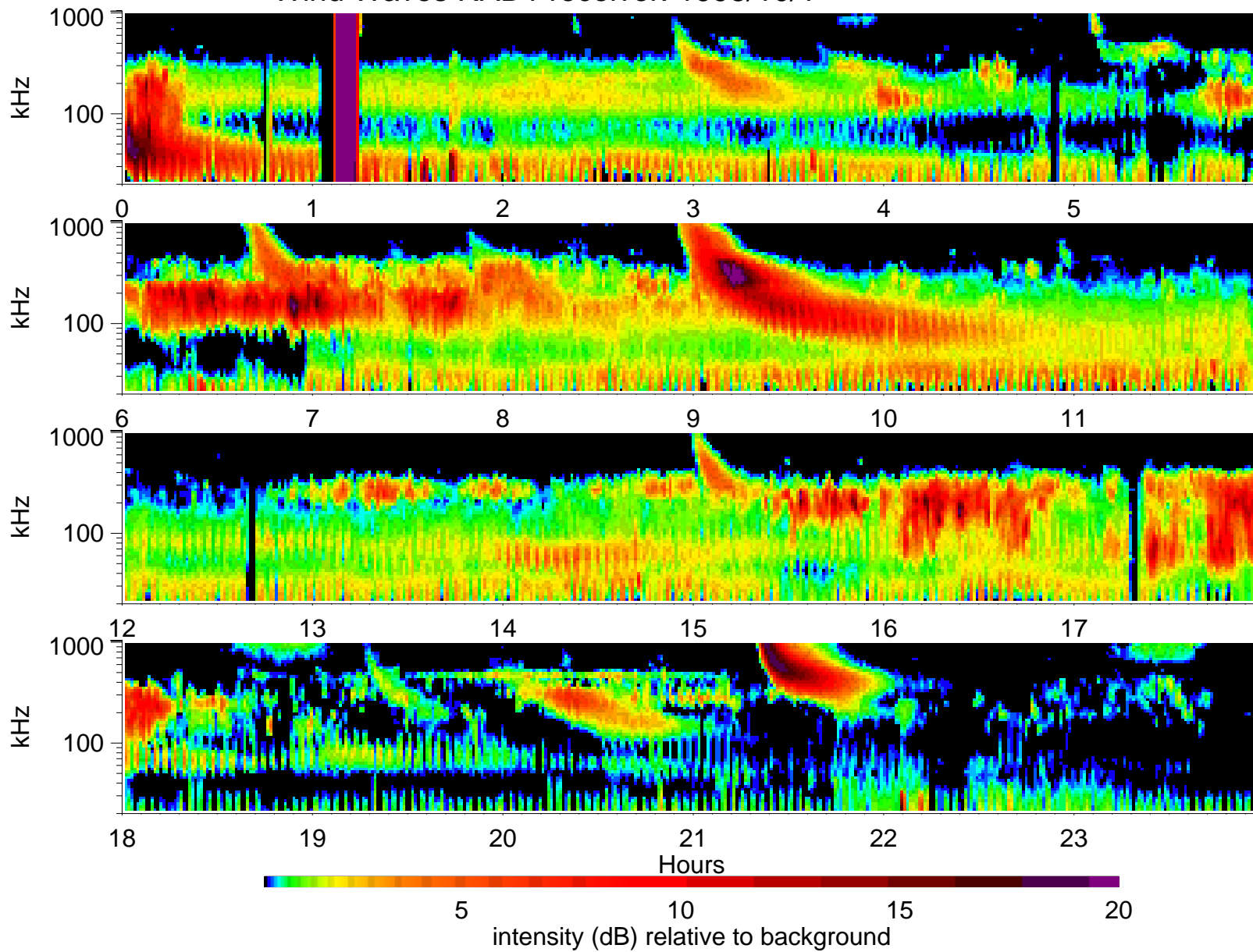
Wind Waves RAD1 receiver: 1998/10/1
