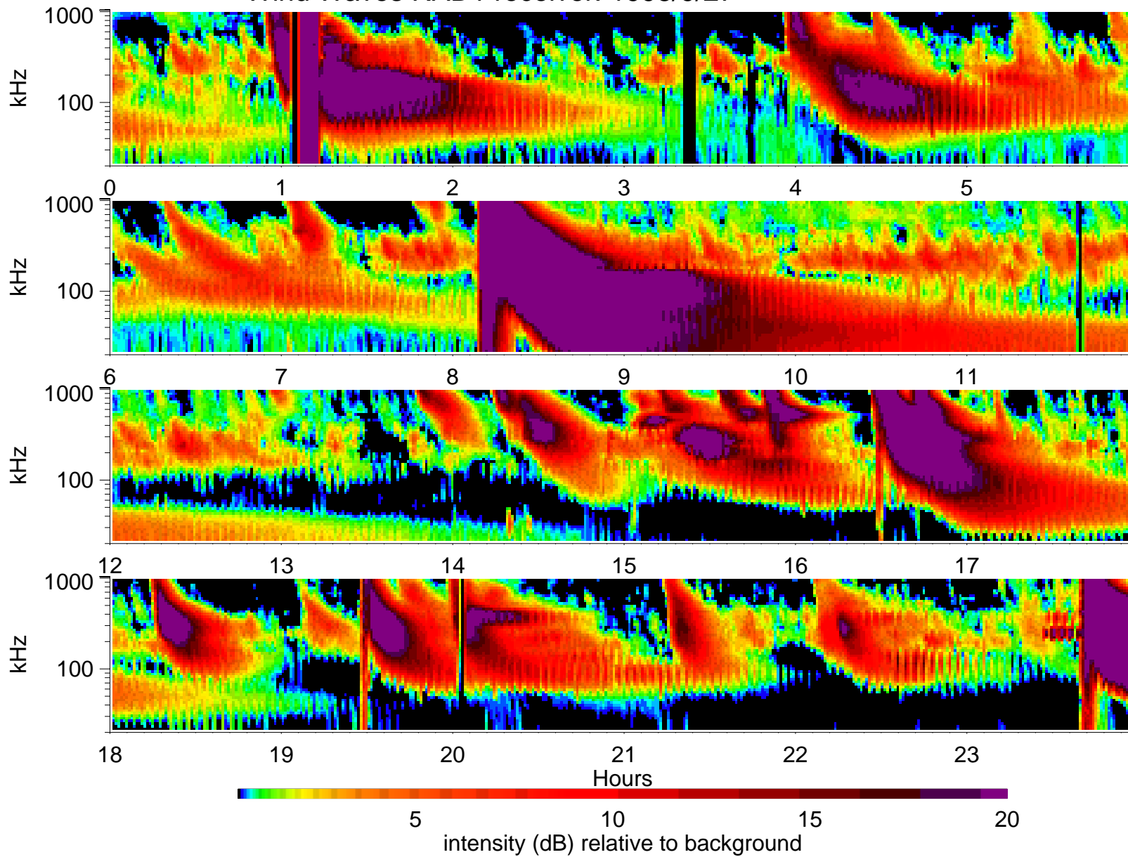
Wind Waves RAD1 receiver: 1998/9/27
