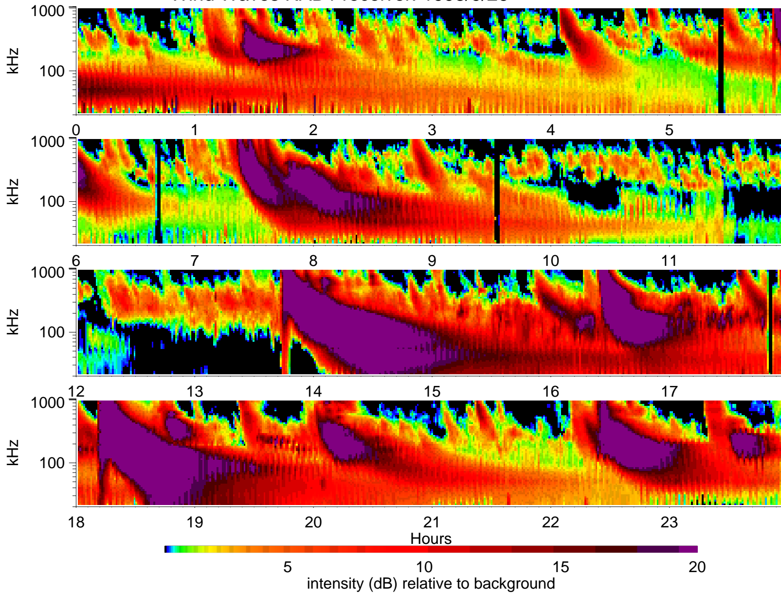
Wind Waves RAD1 receiver: 1998/9/26
