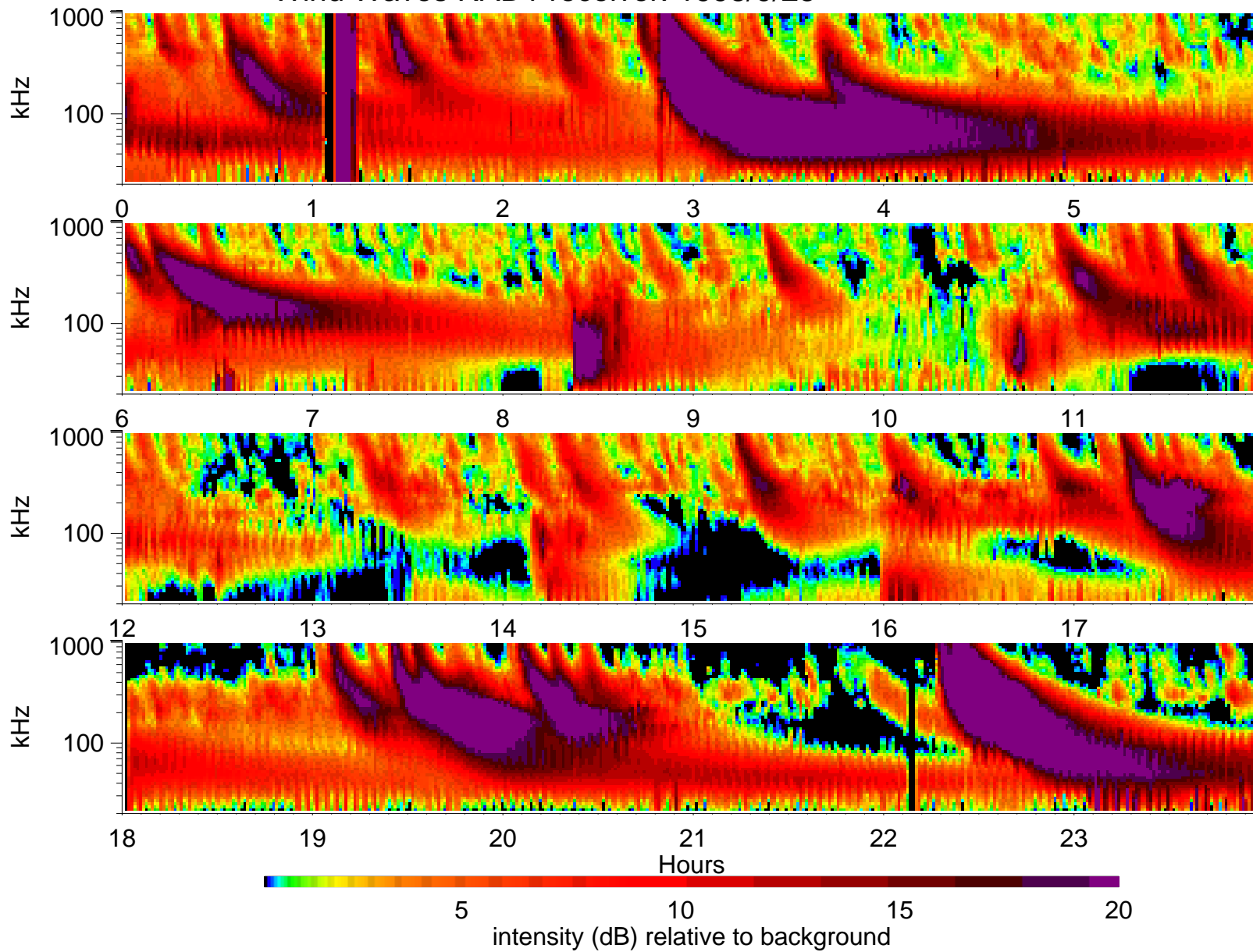
Wind Waves RAD1 receiver: 1998/9/25
