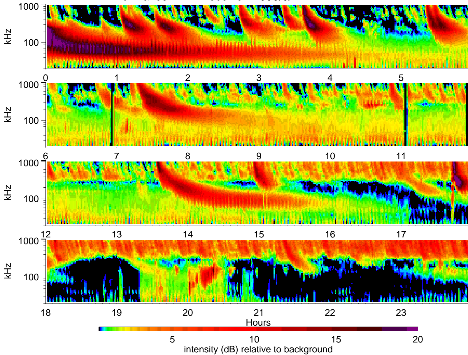
Wind Waves RAD1 receiver: 1998/9/22
