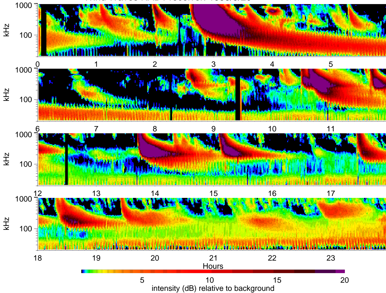
Wind Waves RAD1 receiver: 1998/9/20
