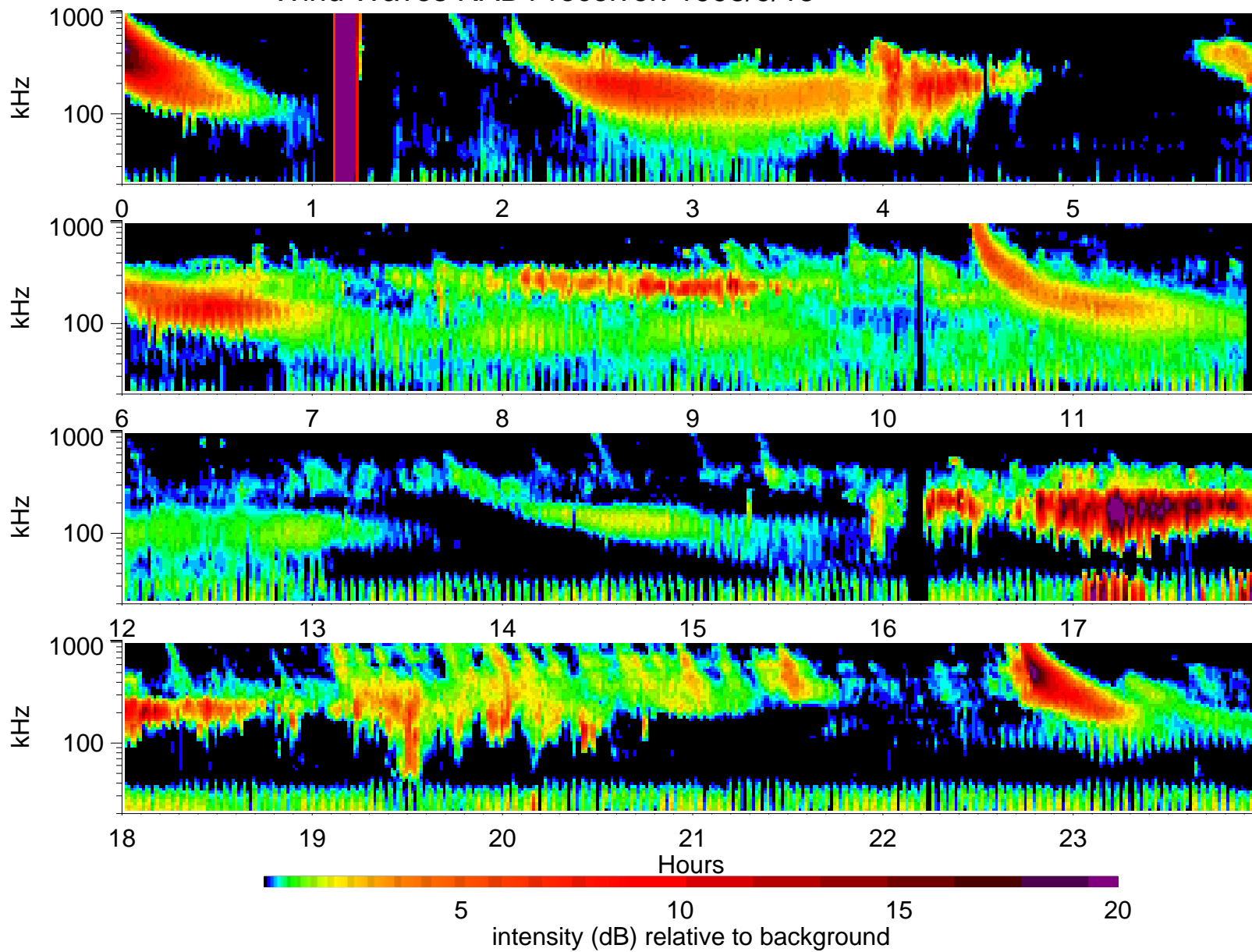
Wind Waves RAD1 receiver: 1998/9/15
