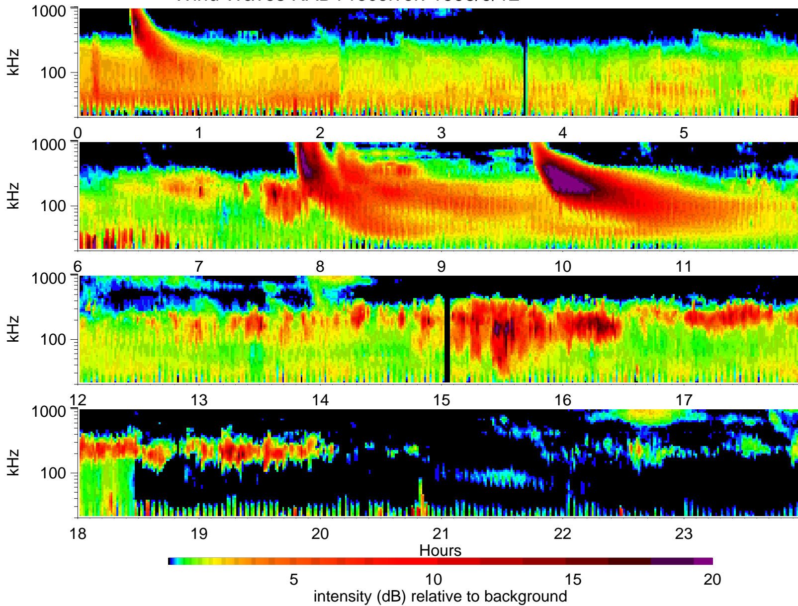
Wind Waves RAD1 receiver: 1998/9/12
