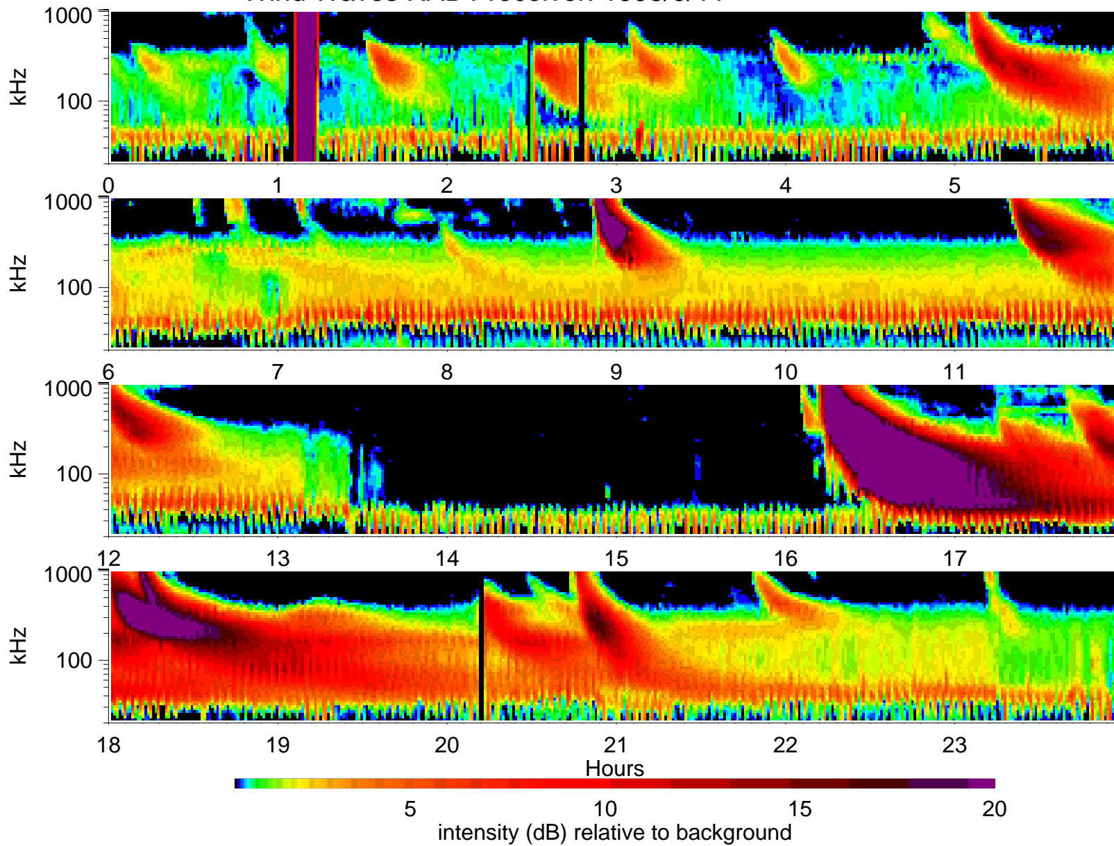
Wind Waves RAD1 receiver: 1998/9/11
