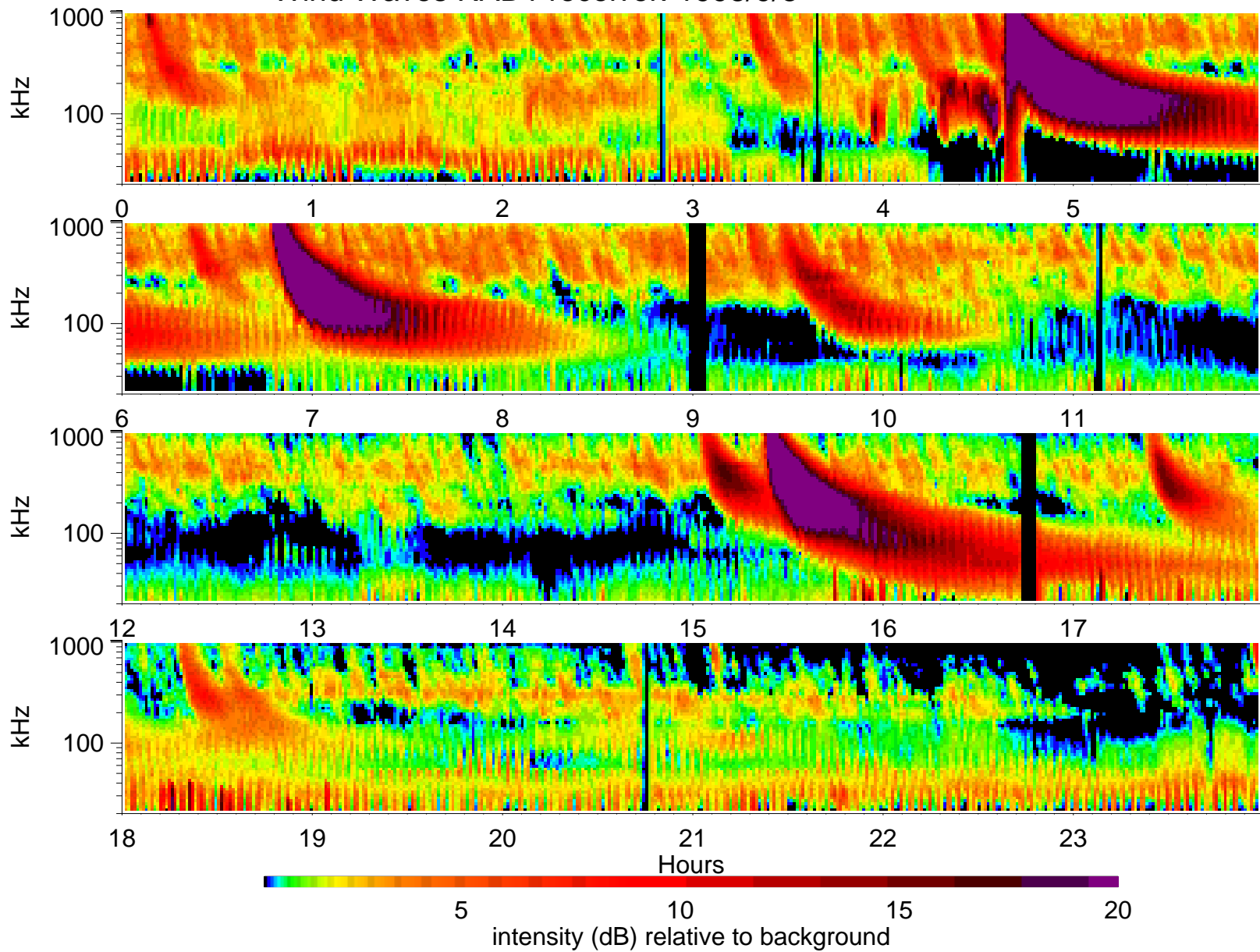
Wind Waves RAD1 receiver: 1998/9/8
