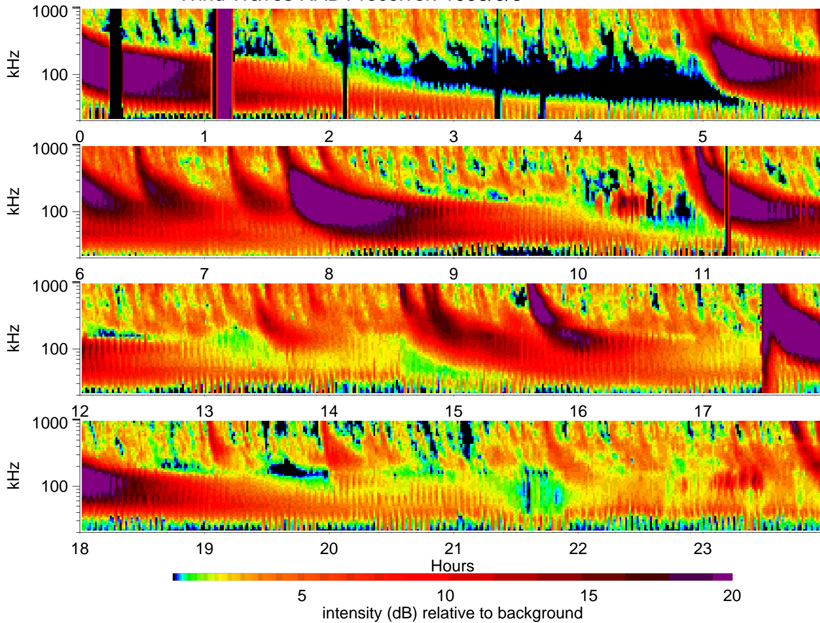
Wind Waves RAD1 receiver: 1998/9/5
