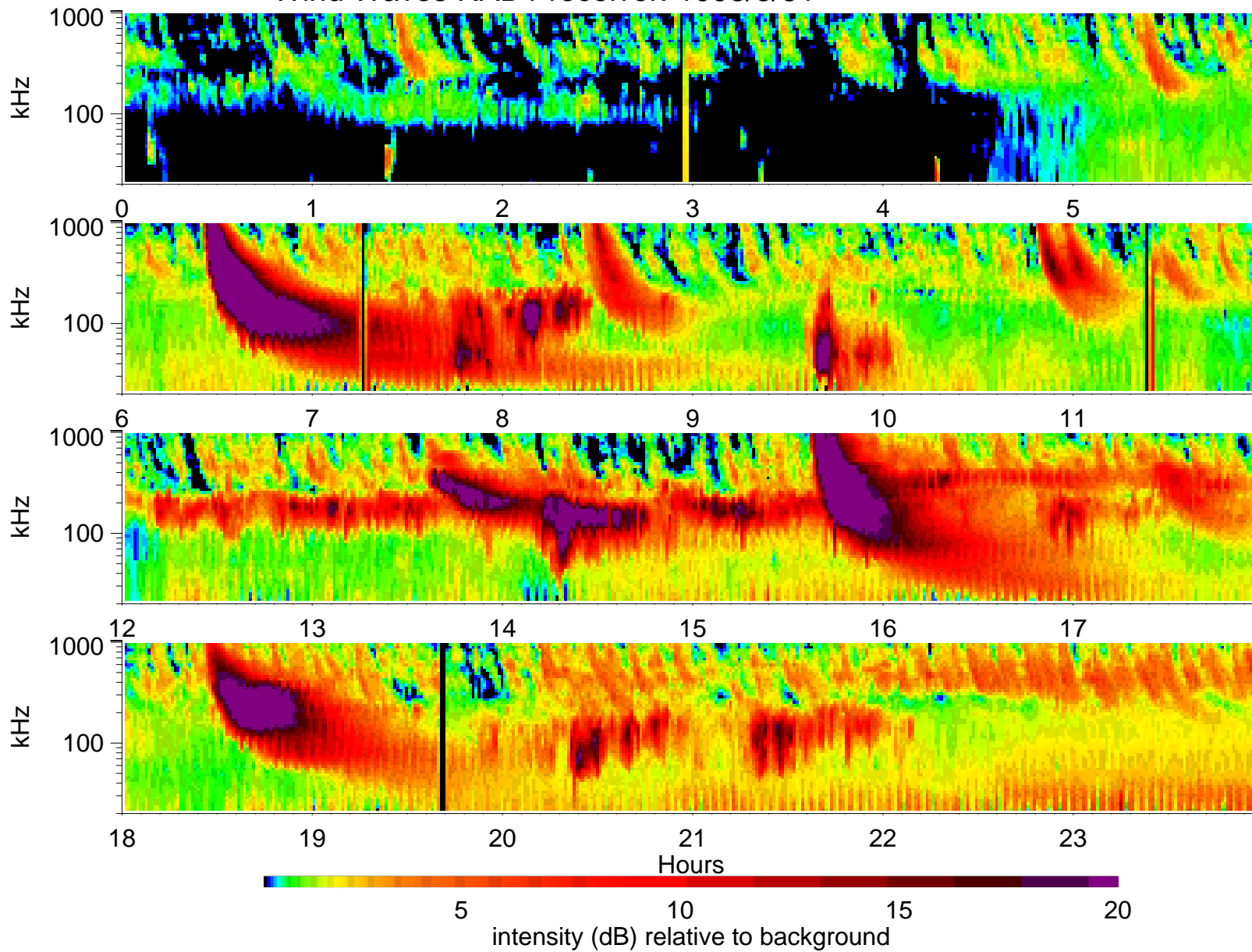
Wind Waves RAD1 receiver: 1998/8/31
