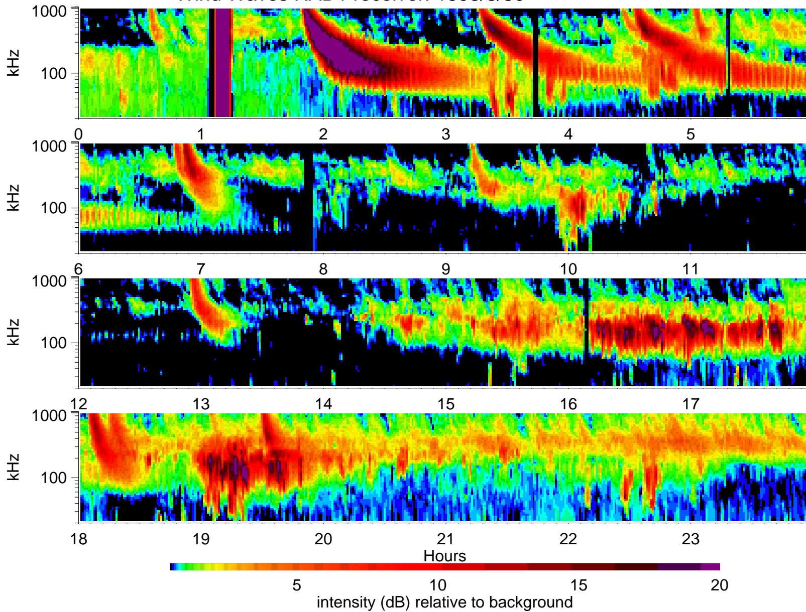
Wind Waves RAD1 receiver: 1998/8/30
