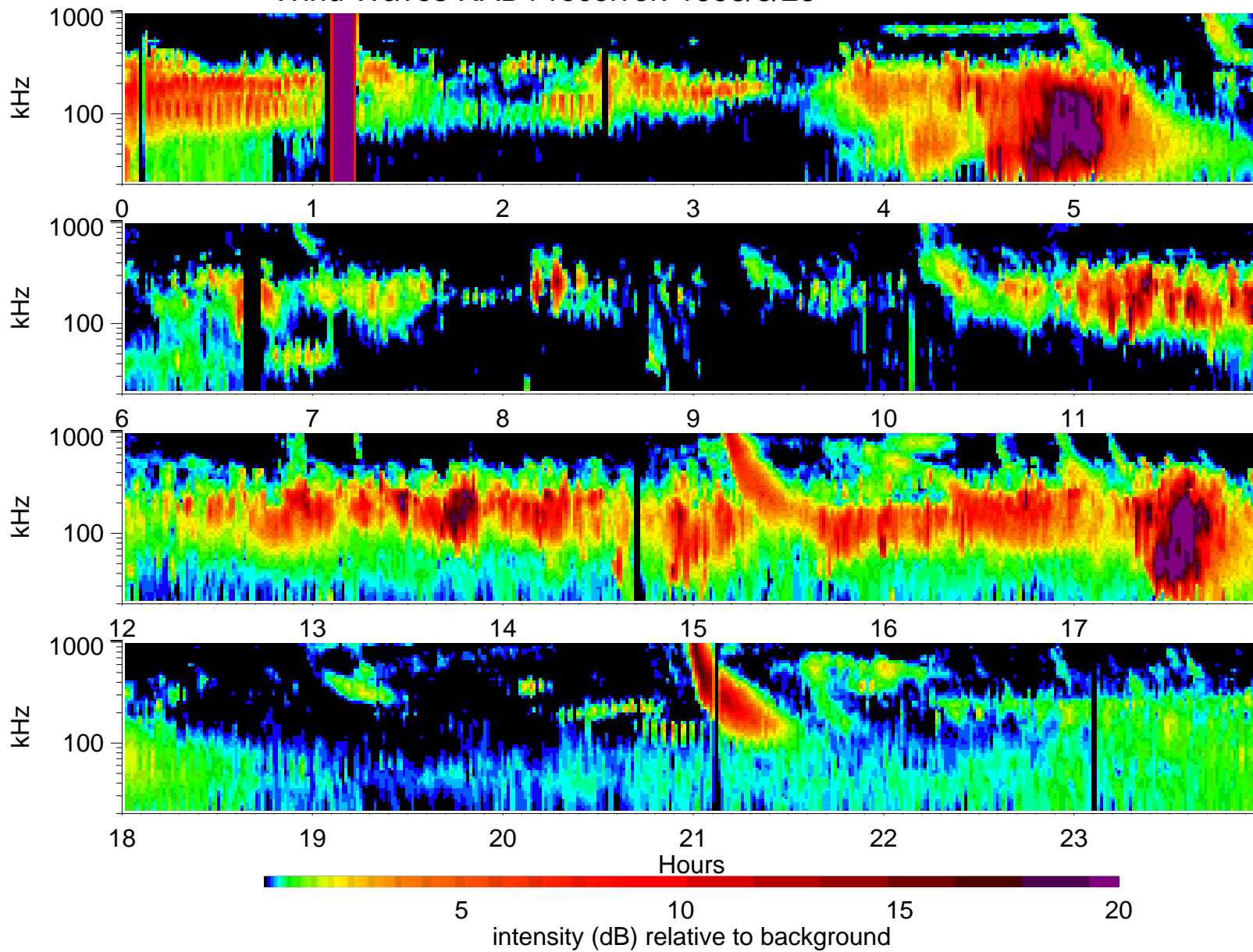
Wind Waves RAD1 receiver: 1998/8/28
